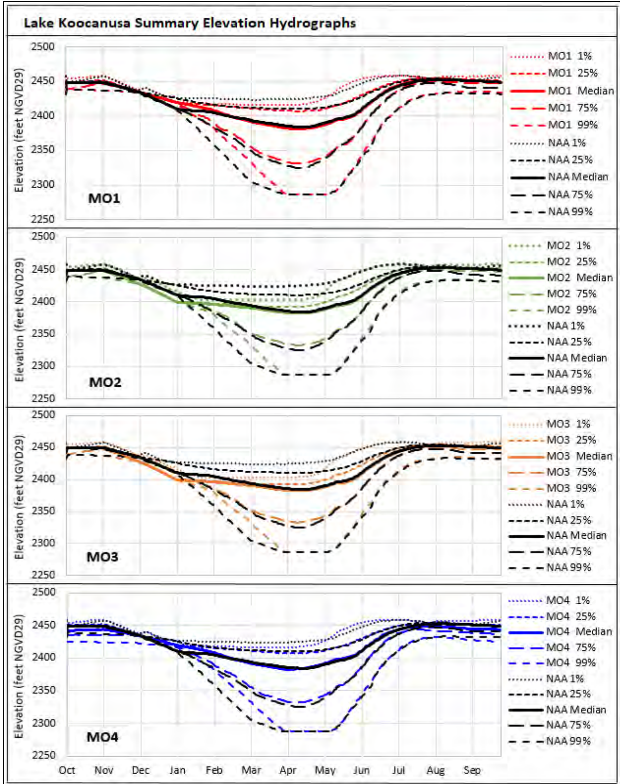
Figure 5-14. Summary Elevation Hydrographs at Libby Reservoir (Lake Kooconusa)
