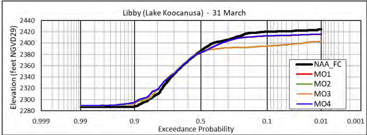
Figure 5-21. Elevation-Frequency Curves for March 31 at Libby Reservoir (Lake Kocanusa)
