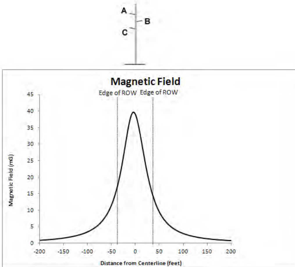
FIGURE 4.16-7 CASE II: SINGLE POLE VERTICAL CIRCUIT-MAGNETIC FIELD
