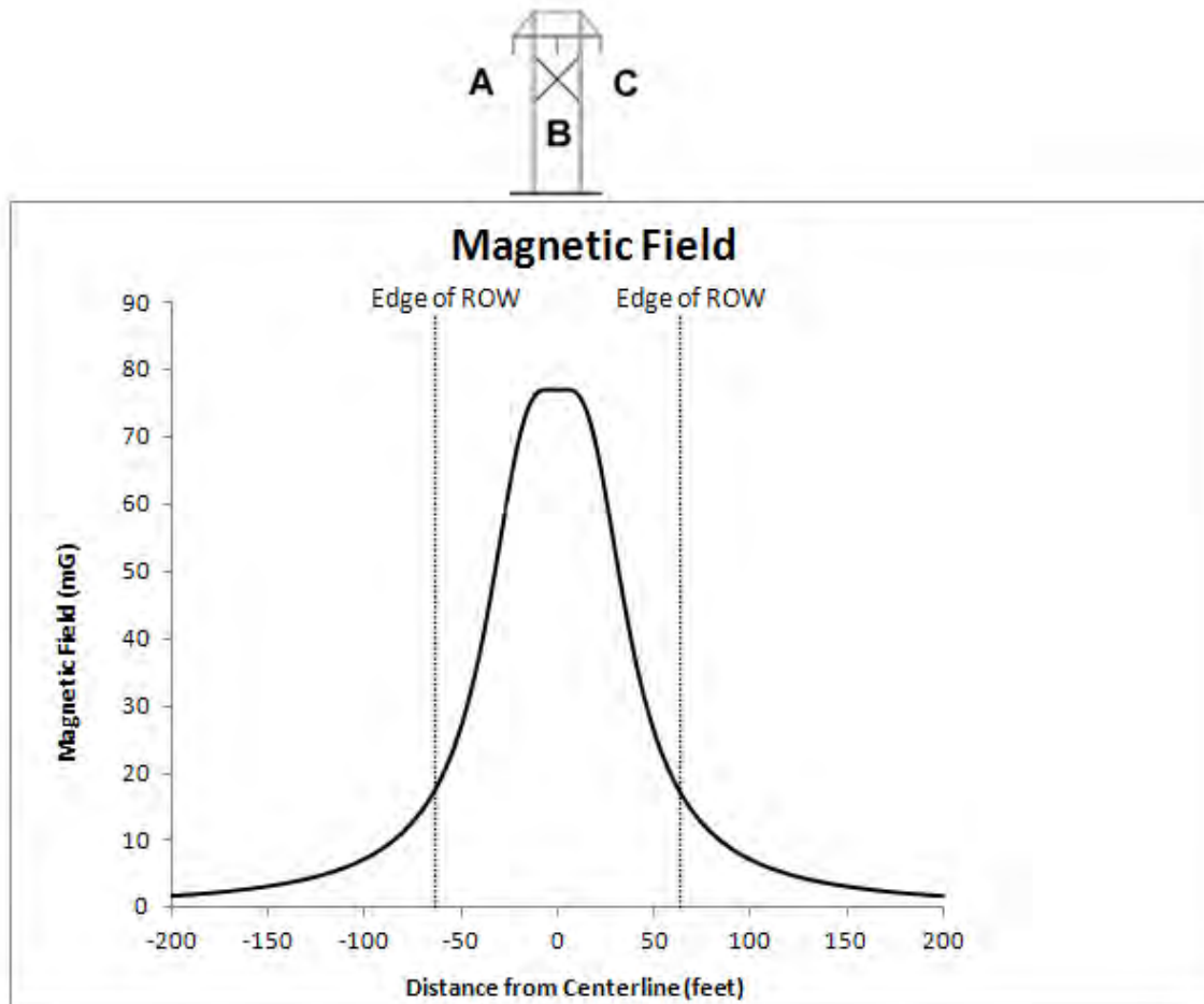
FIGURE 4.16-6 CASE I: H-FRAME HORIZONTAL CIRCUIT-MAGNETIC FIELD
