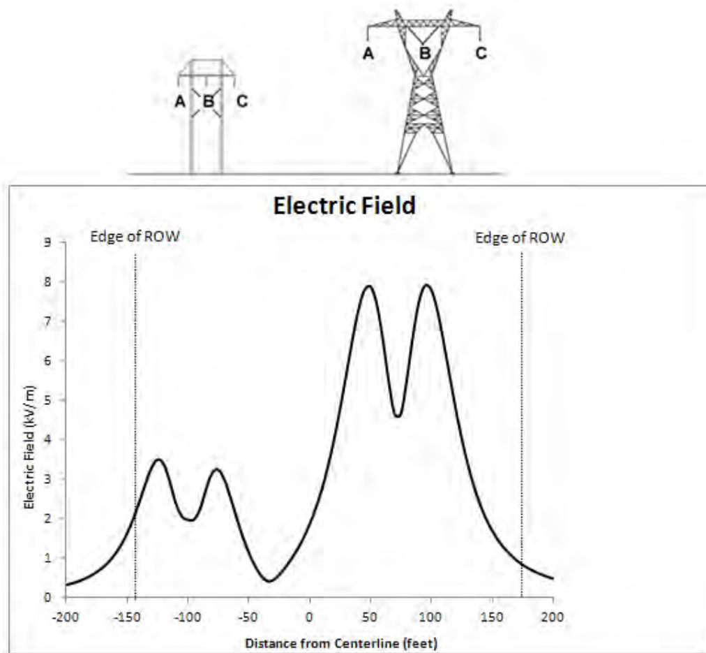
FIGURE 4.16-5 CASE V: H-FRAME PARALLEL TO BPA HANFORD-VANTAGE 500 KV - ELECTRIC FIELD
