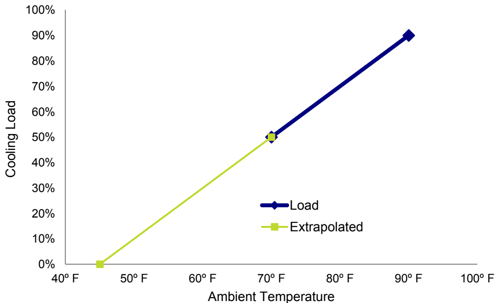
Figure 3.1: Example Extrapolation of Cooling Load by Ambient Temperature
