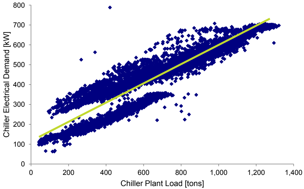
Figure 3.4: Example of Inaccurate Regression Prediction of Chiller Demand
