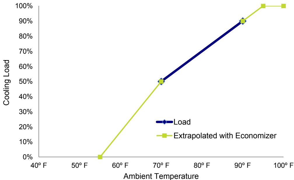
Figure 3.2: Example Extrapolated Cooling Load with Economizer
