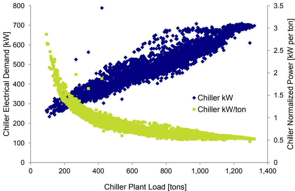
Figure 3.3: Examples of Demand and Power Graphed Against Chiller Load
