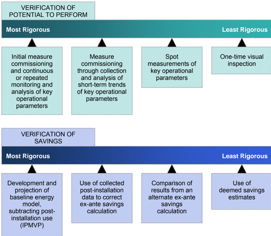
Figure 2.1: Spectrum of Rigor Levels in Savings Verification
