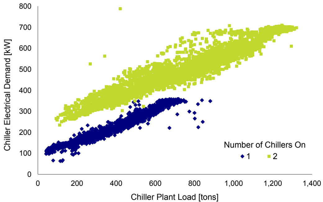
Figure 3.5: Example of Appropriate Interpretation of Data from Multiple Chillers
