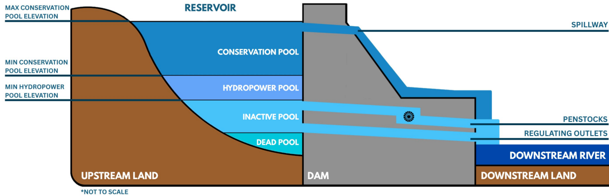
Figure 2-2. Conceptual Cross Section of a Hydropower Power Dam Showing the Vertical Layout of the Outlets and Pool Designations.
