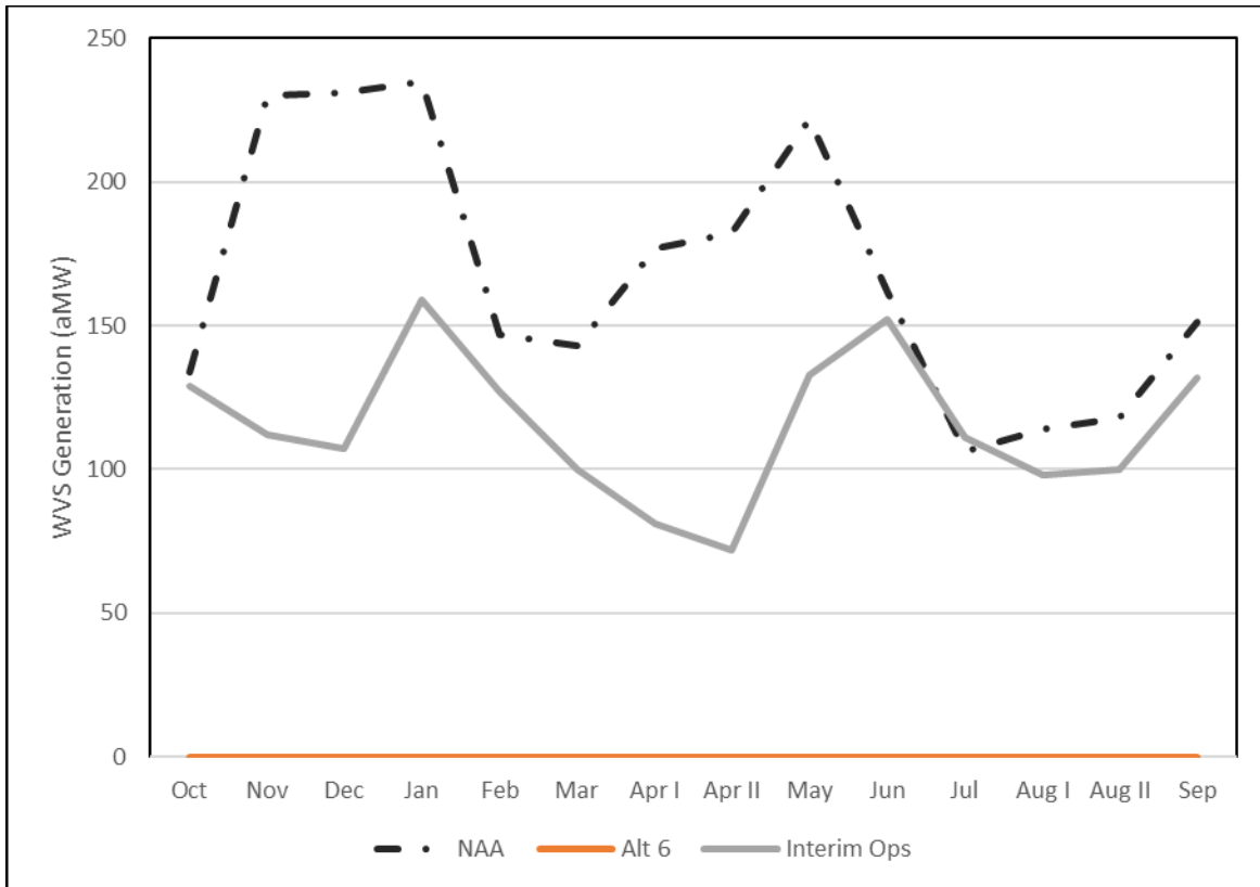
Figure 3-32. Monthly Average Generation (aMW) under the No-action Alternative, Alternative 6, and Interim Operations.
