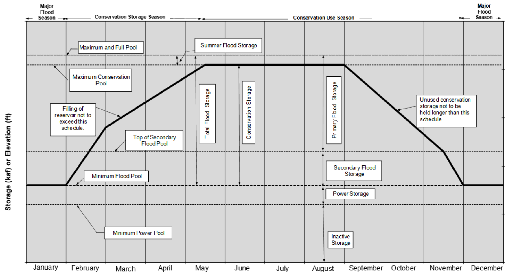
Figure 1-1. Typical Water Control Diagram for WVS Dams and Reservoirs.
