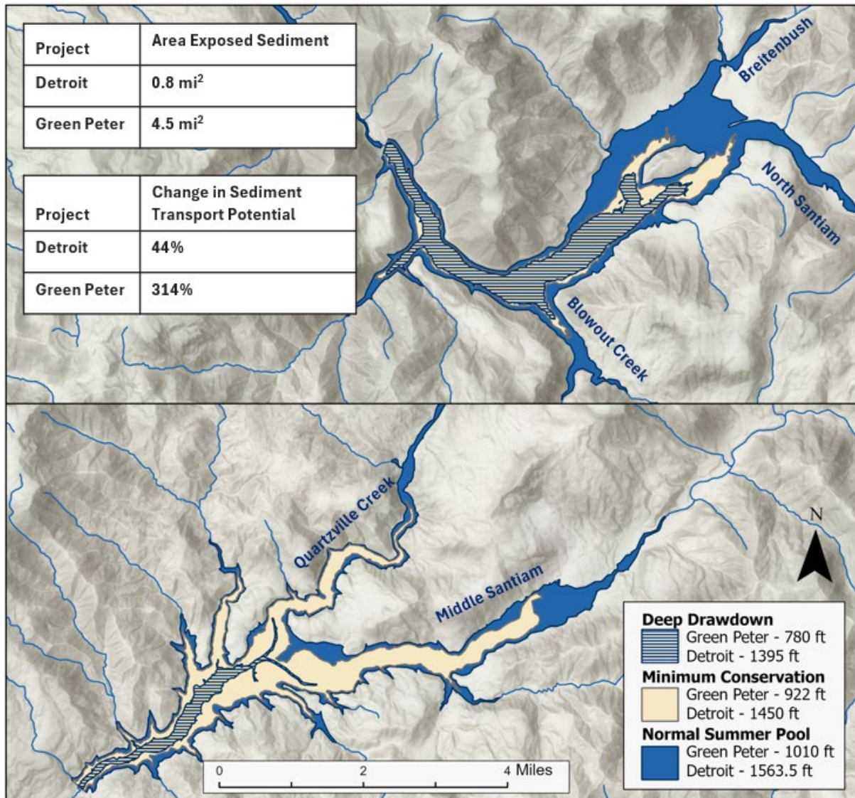
Figure 3-33. Green Peter (bottom) and Detroit (top) Exposed Areas between the Normal Minimum Conservation Pool and the Deep Drawdown Elevations.
