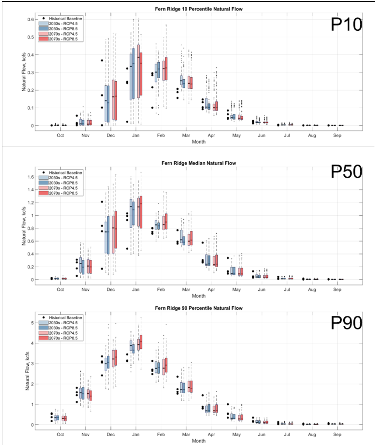
Figure 6-7. Fern Ridge Dam and Reservoir Climate Change Projections.
