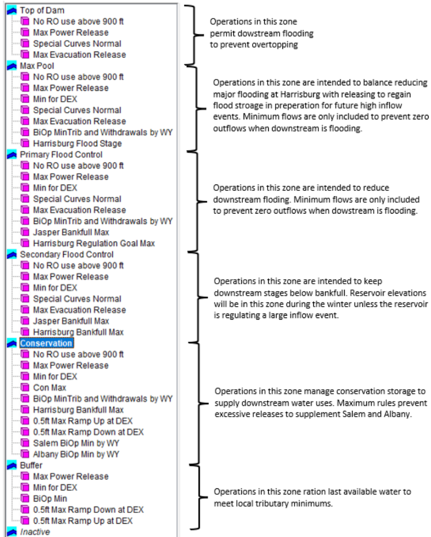
Figure 3-37. Lookout Point Dam and Reservoir Operational Summary.
