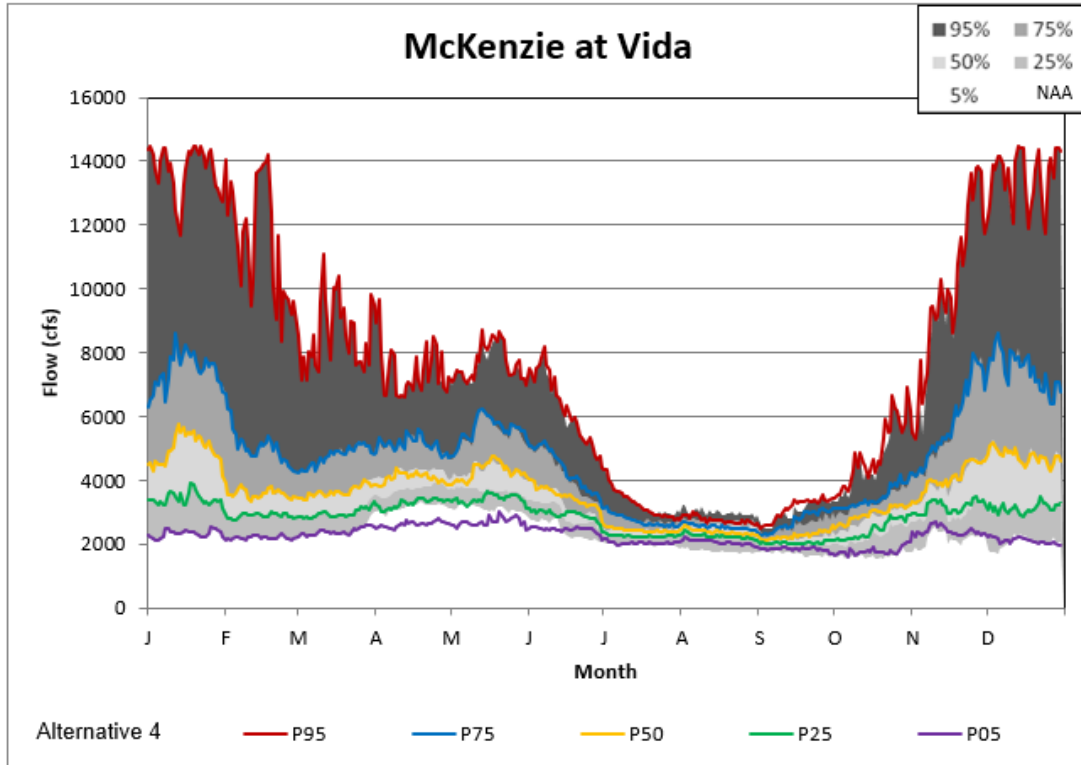
Figure 5-132. Vida Alternative 4 Non-exceedance Plot.
