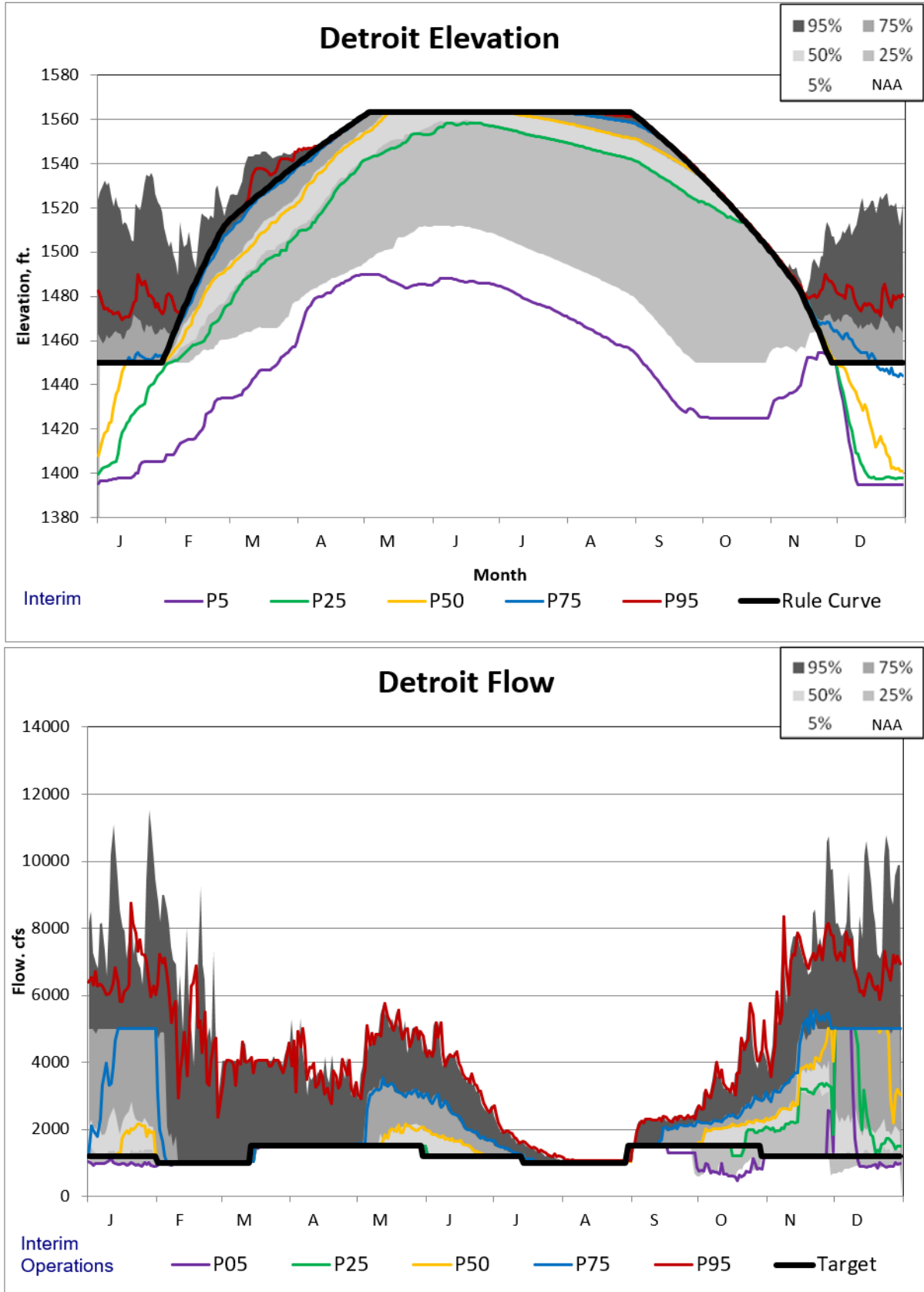
Figure 5-213. Detroit Updated Interim Operations Non-exceedance Plot.
