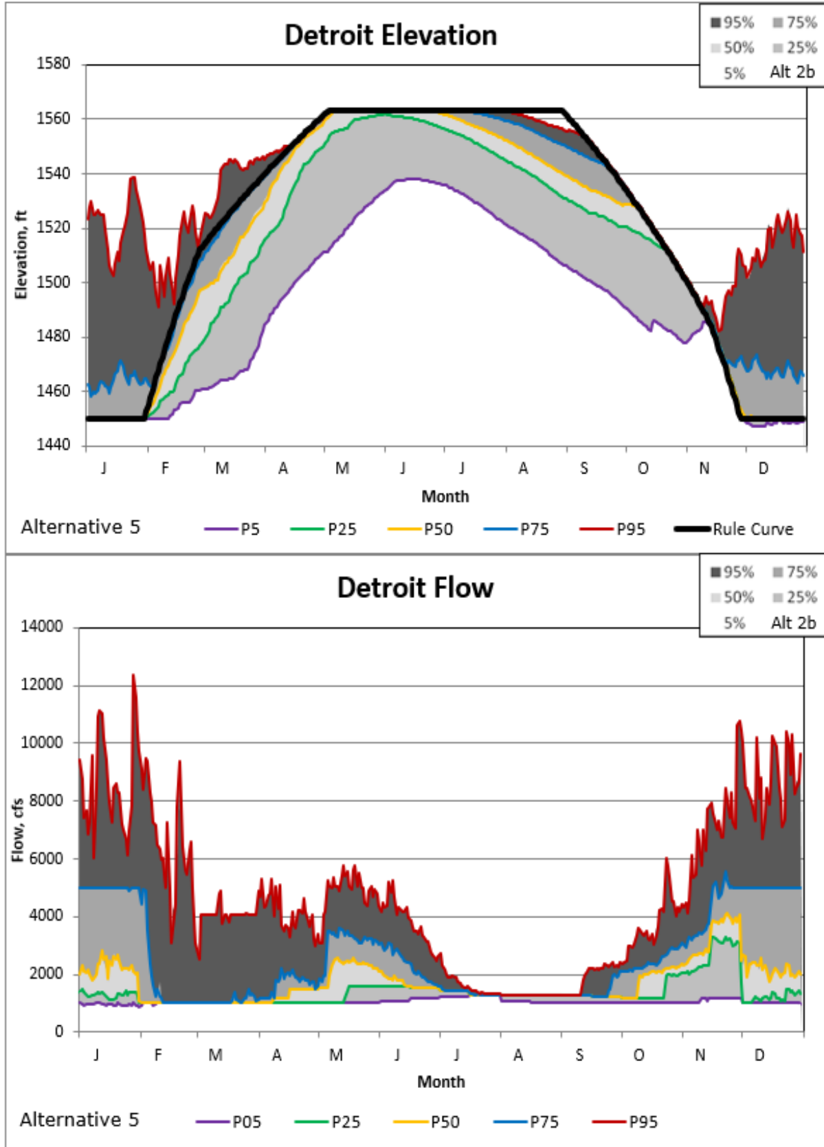
Figure 5-236. Detroit Alternatives 5/2B Non-exceedance Plot.
