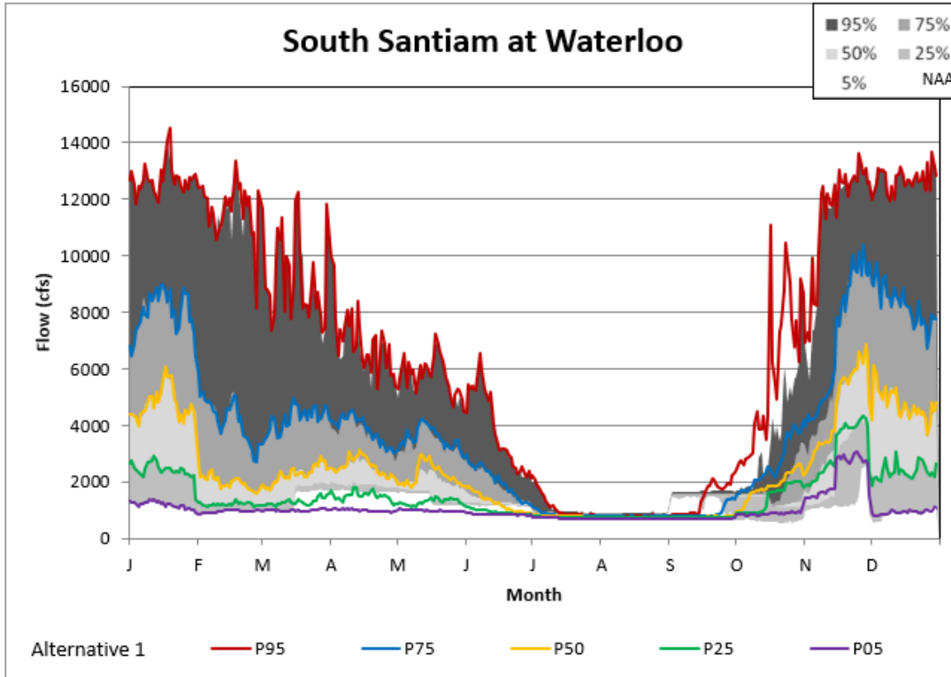
Figure 5-21. Waterloo Alternative 1 Non-exceedance Plot.
