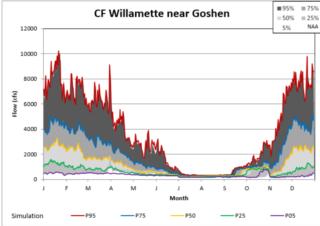
Figure-5-15. Goshen Alternative 1 Non-Exceedance Plot.
