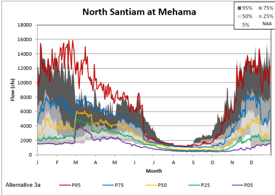
Figure 5-88. Mehama Alternative 3A Non-exceedance Plot.
