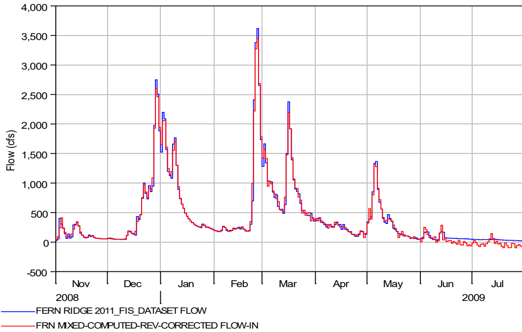
Figure 2-23. Water Year 2009 Comparison at Fern Ridge Reservoir.
