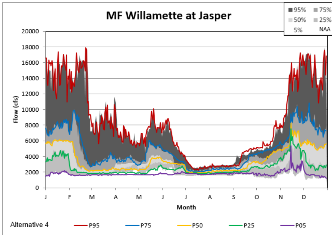
Figure 5-133. Jasper Alternative 4 Non-exceedance Plot.
