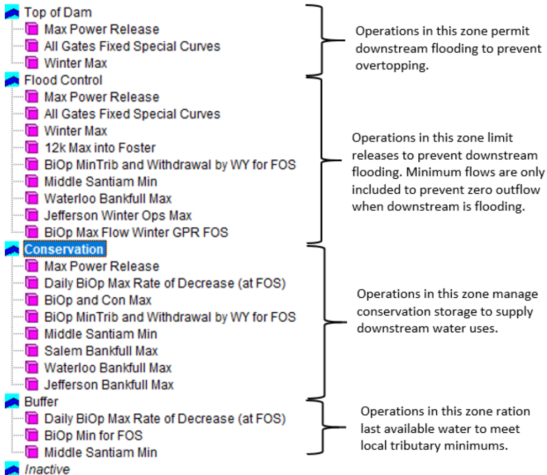
Figure 3-45. Green Peter Dam and Reservoir Operational Summary.
