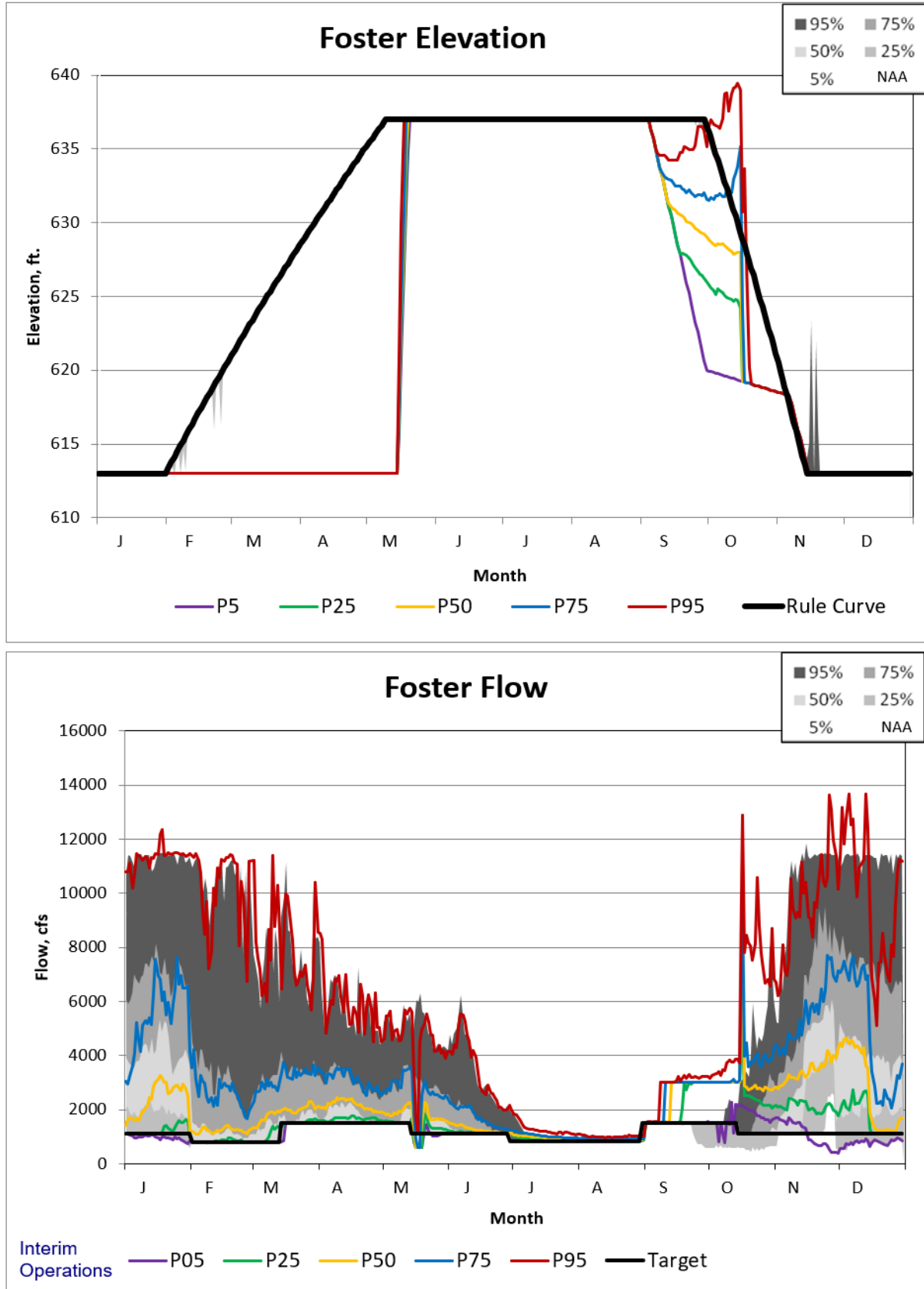
Figure 5-218. Foster Updated Interim Operations Non-exceedance Plot.
