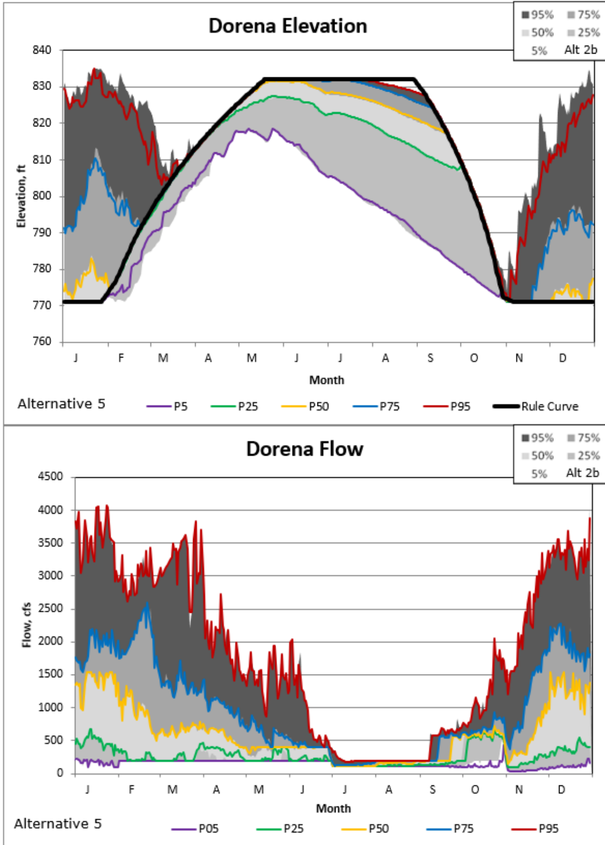
Figure 5-238. Dorena Alternatives 5/2B Non-exceedance Plot.
