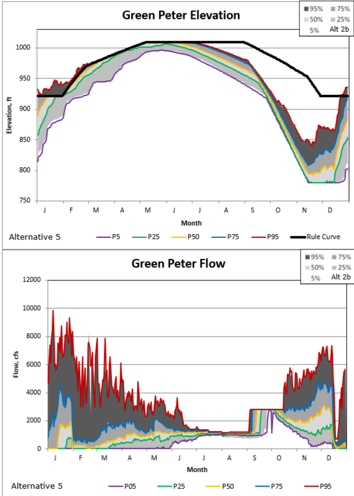
Figure 5-242. Green Peter Alternatives 5/2B Non-exceedance Plot.
