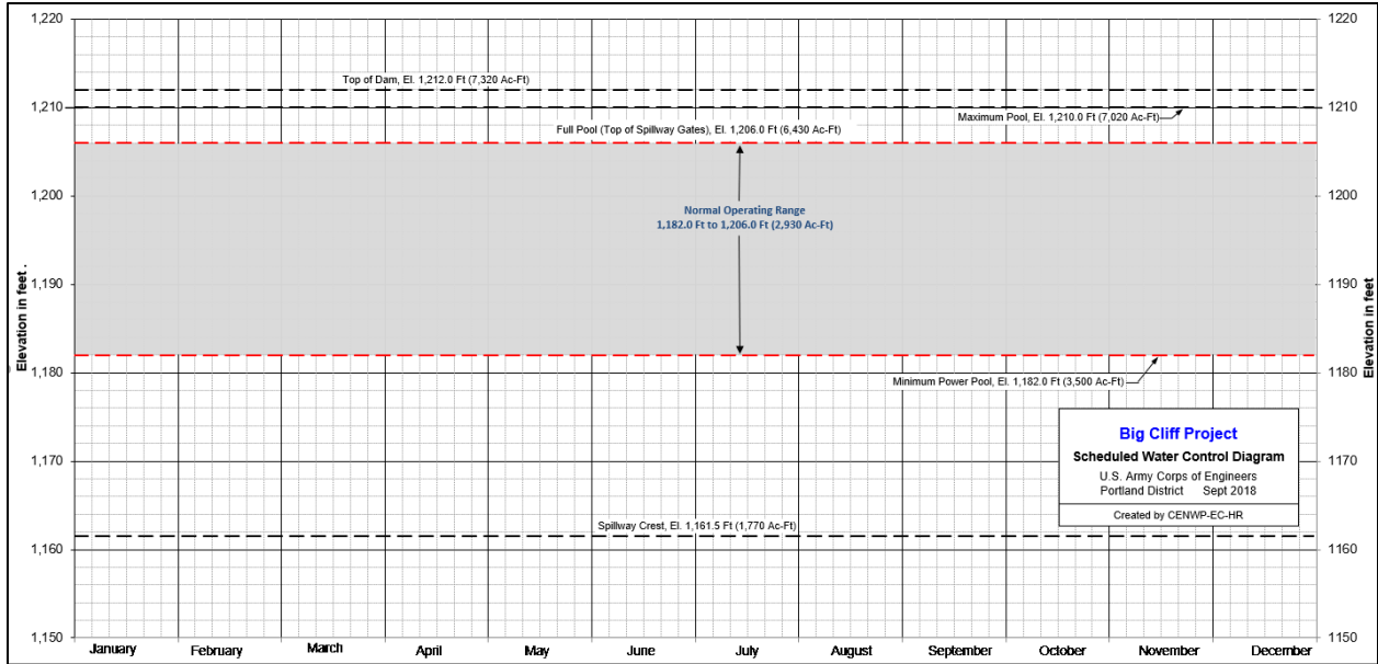
Figure 10-12. Big Cliff Dam and Reservoir Water Control Diagram.
