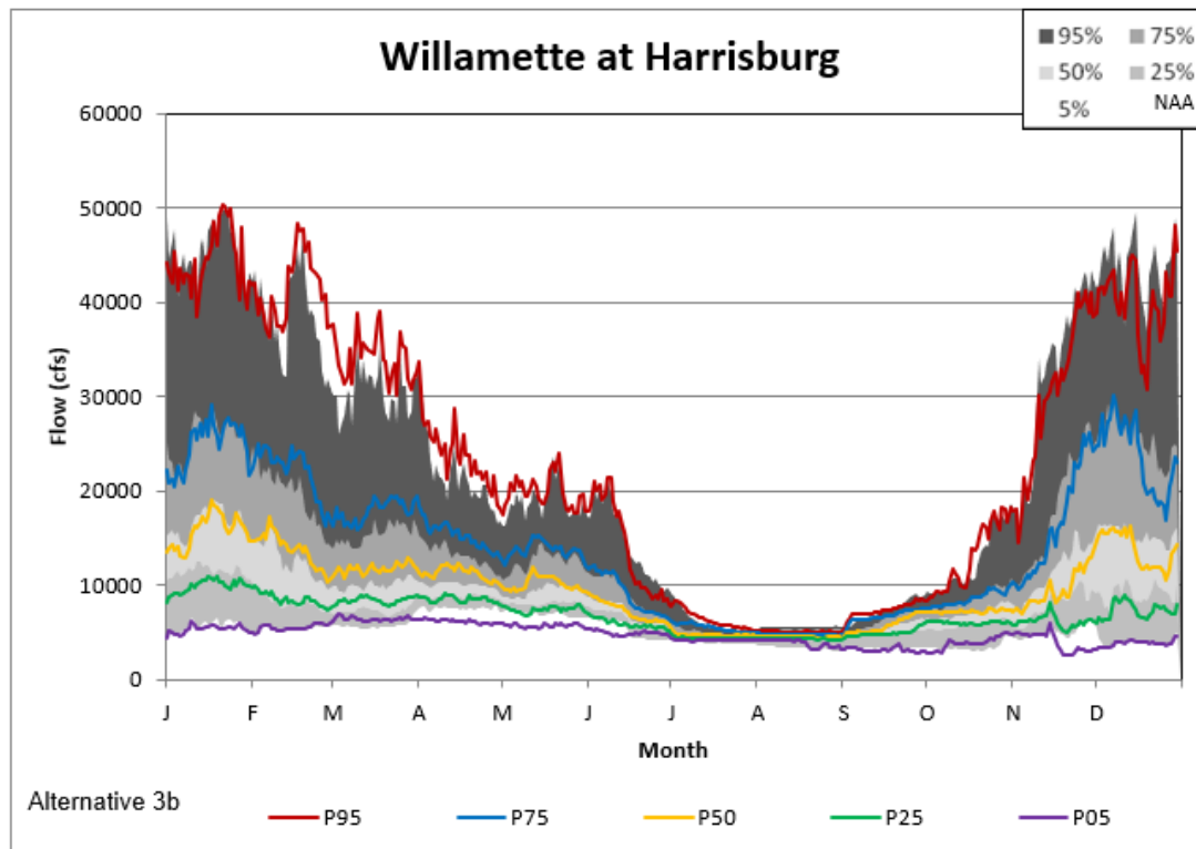
Figure 5-114. Harrisburg Alternative 3B Non-exceedance Plot.
