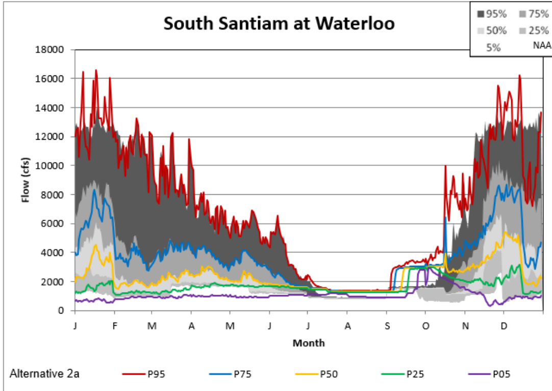
Figure 5-44. Waterloo Alternative 2A Non-exceedance Plot.
