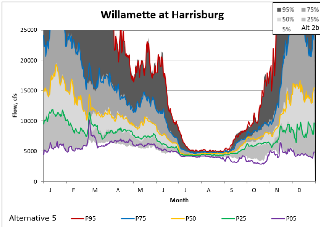
Figure 5-252. Harrisburg Alternatives 5/2B Non-exceedance Plot.
