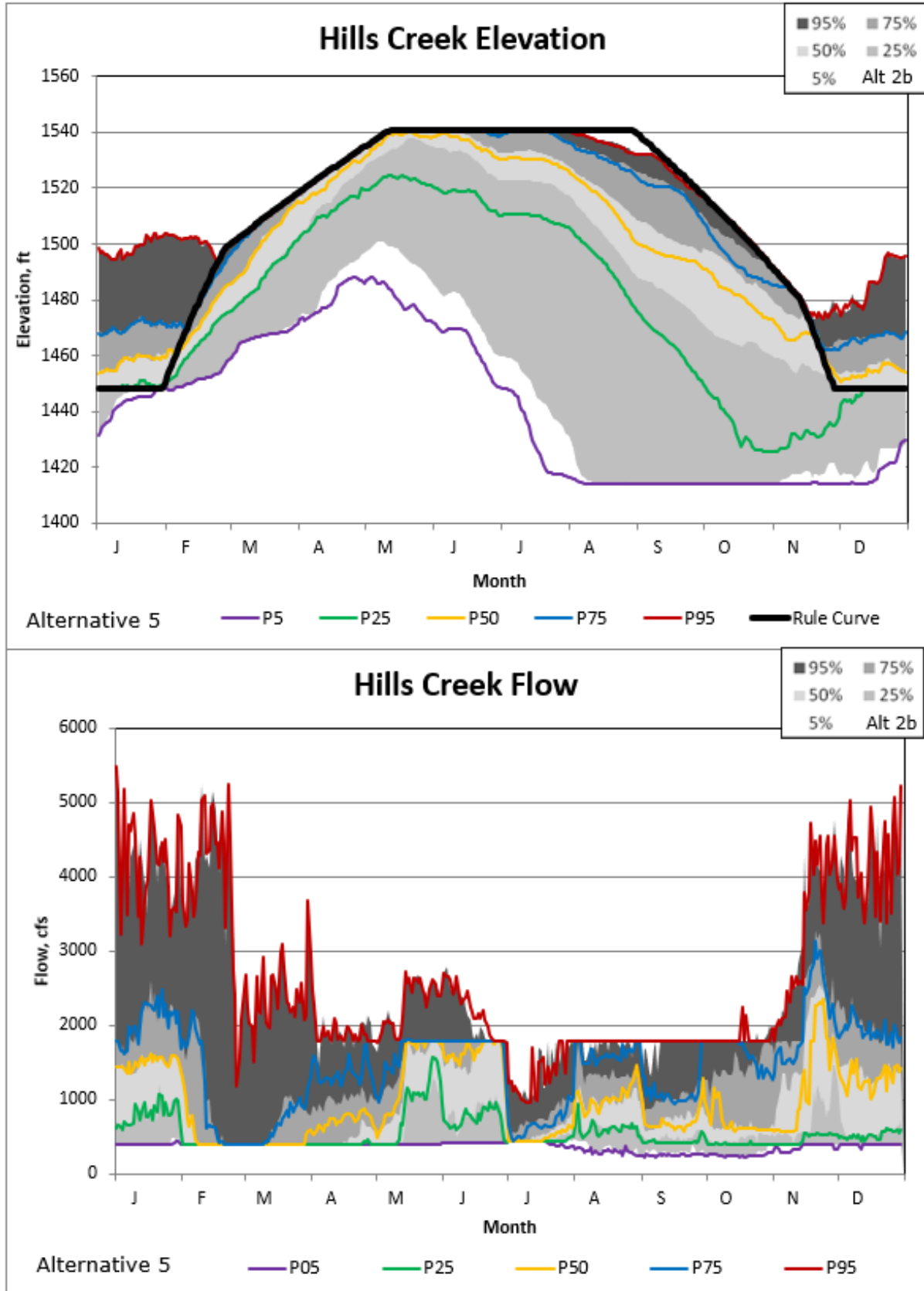
Figure 5-243. Hills Creek Alternatives 5/2B Non-exceedance Plot.
