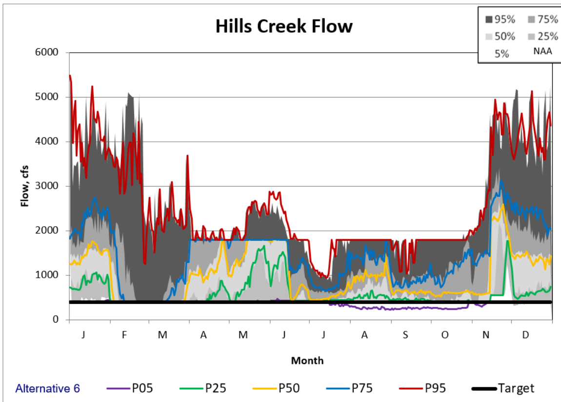
Figure 5-174. Hills Creek Alternative 6 Non-exceedance Plot.
