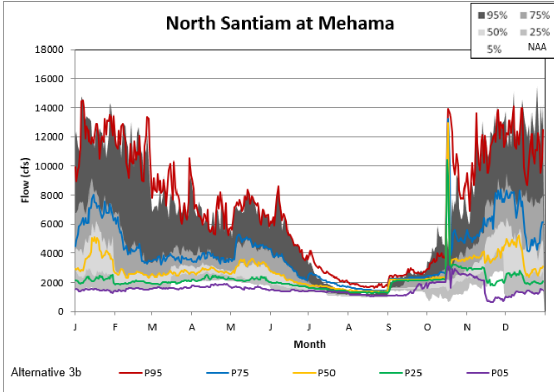
Figure 5-111. Mehama Alternative 3B Non-exceedance Plot.
