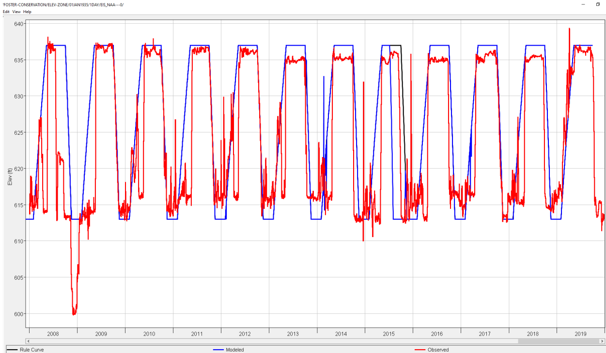
Figure 3-67. Foster Dam and Reservoir Model Validation.
