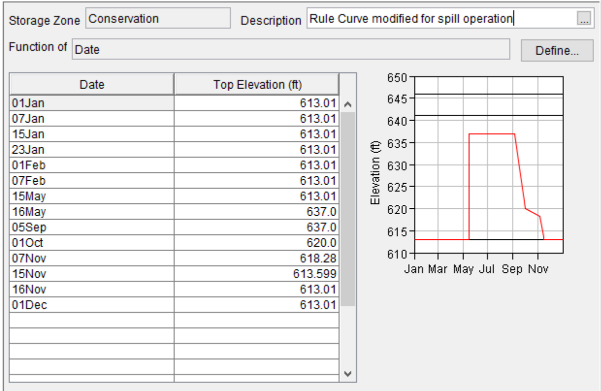
Figure 4-14. Foster Dam and Reservoir Interim Operations Target Elevation.
