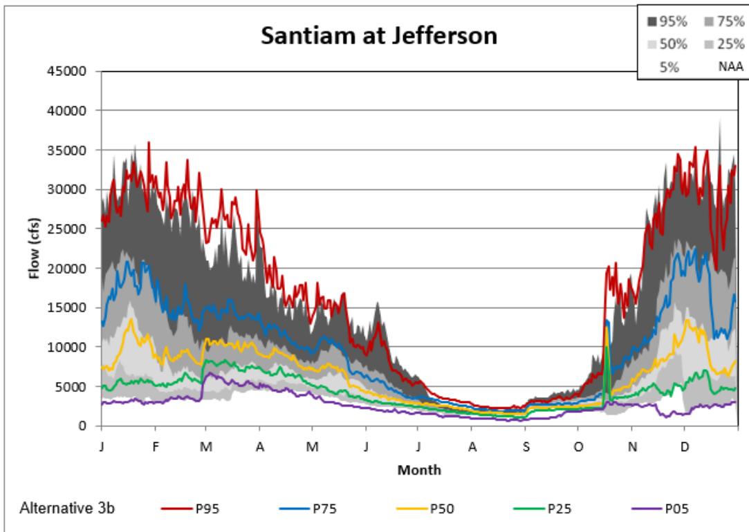
Figure 5-112. Jefferson Alternative 3B Non-exceedance Plot.
