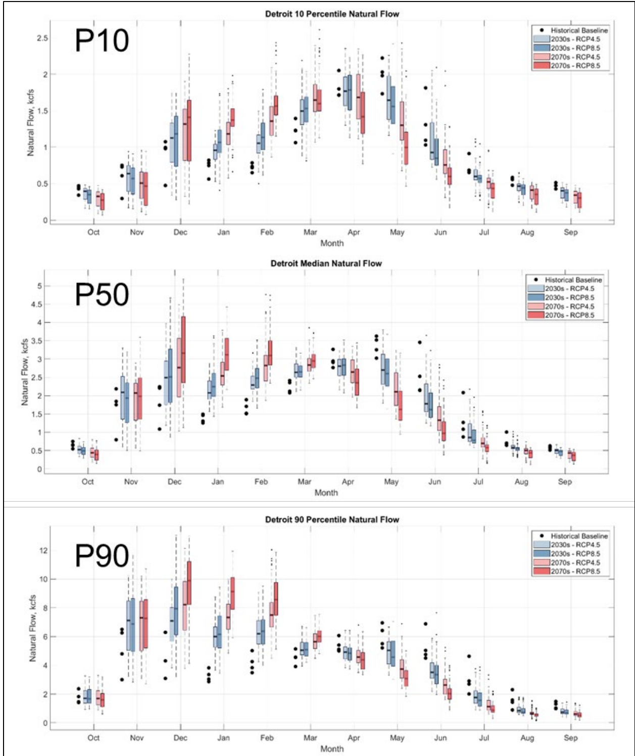
Figure 6-4. Detroit Dam and Reservoir Climate Change Projections.
