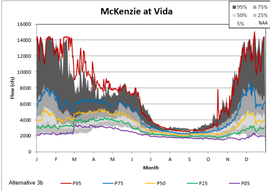
Figure 5-109. Vida Alternative 3B Non-exceedance Plot.
