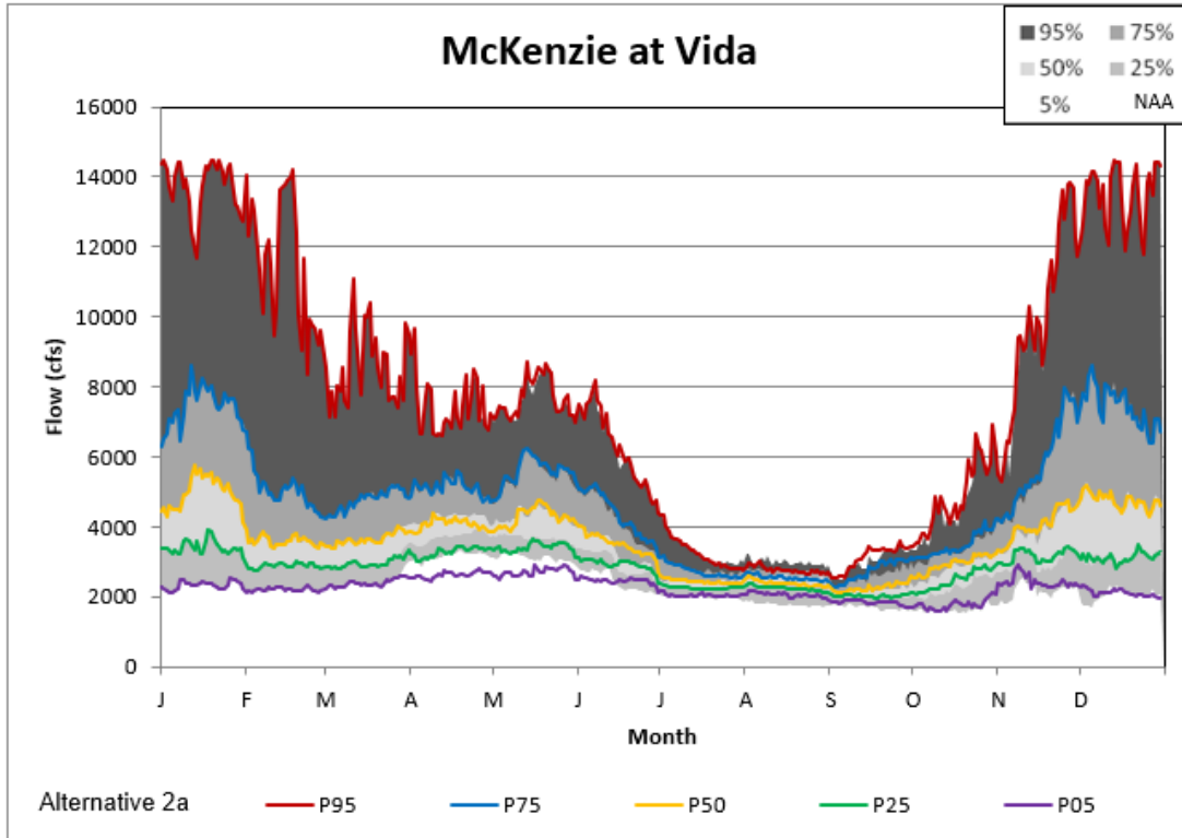
Figure 5-40. Vida Alternative 2A Non-exceedance Plot.
