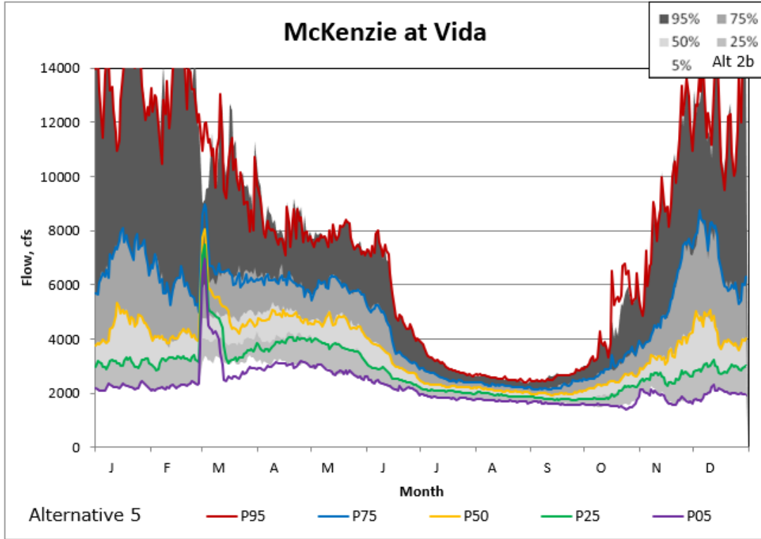
Figure 5-247. Vida Alternatives 5/2B Non-exceedance Plot.
