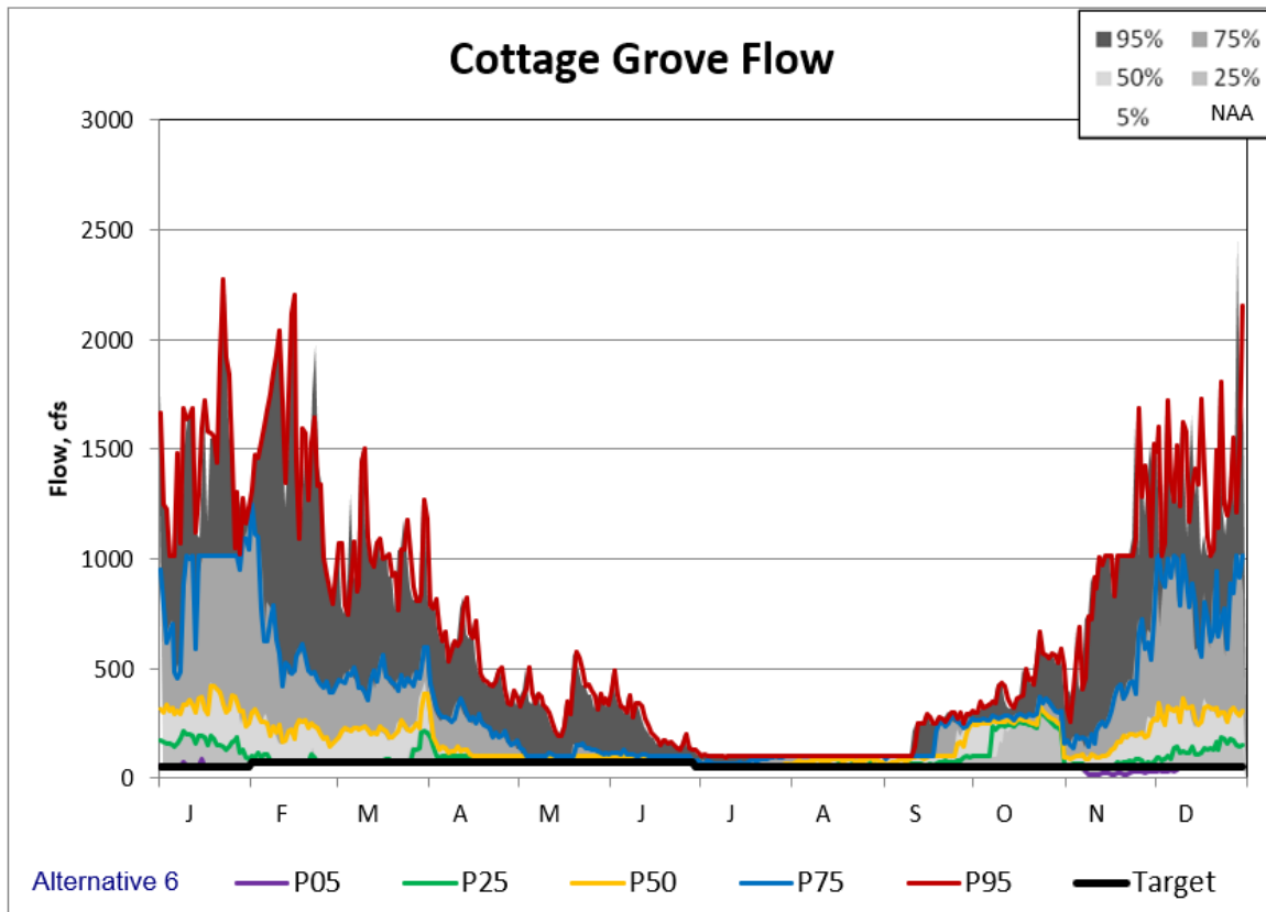
Figure 5-165. Cottage Grove Alternative 6 Non-exceedance Plot.
