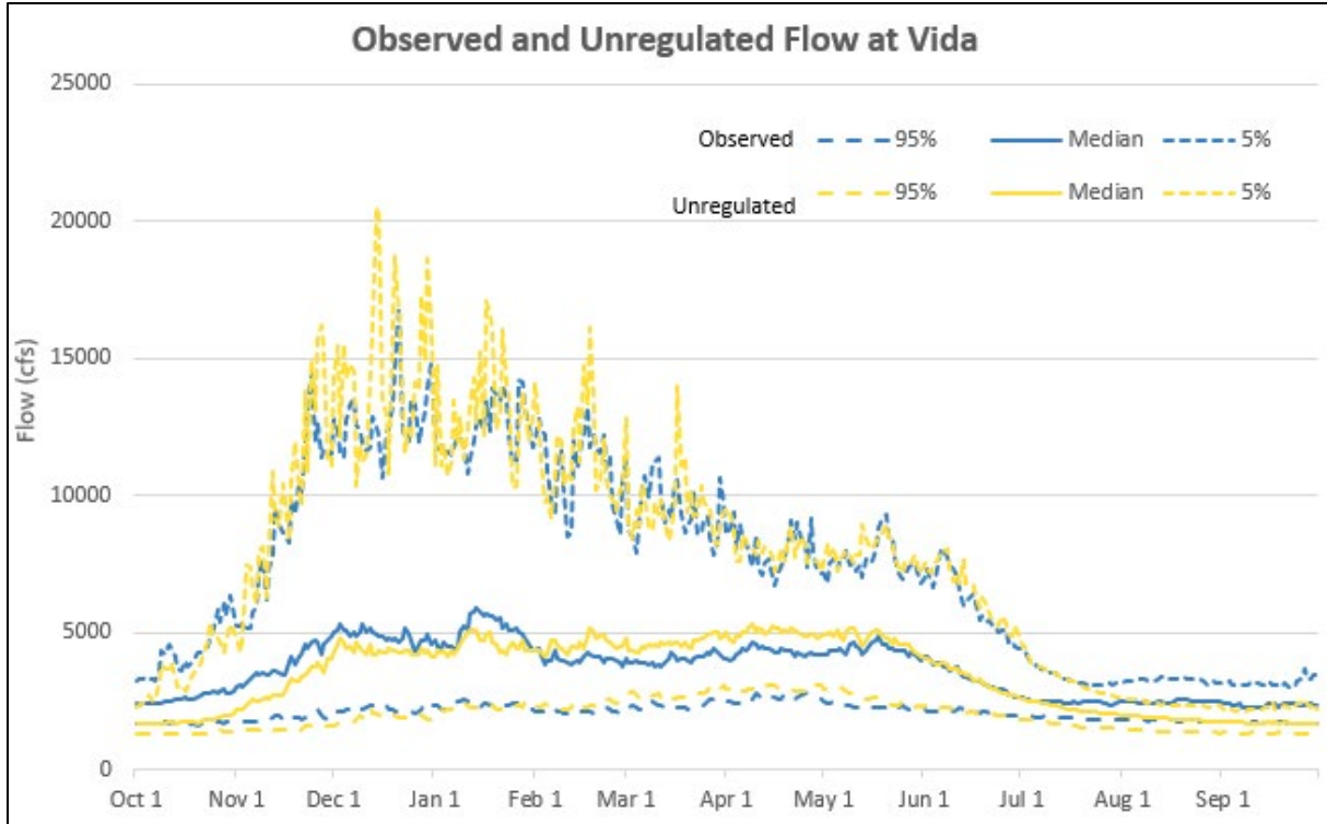
Figure 11-3. McKenzie River at Vida, OR. Flows across the Water Year.
