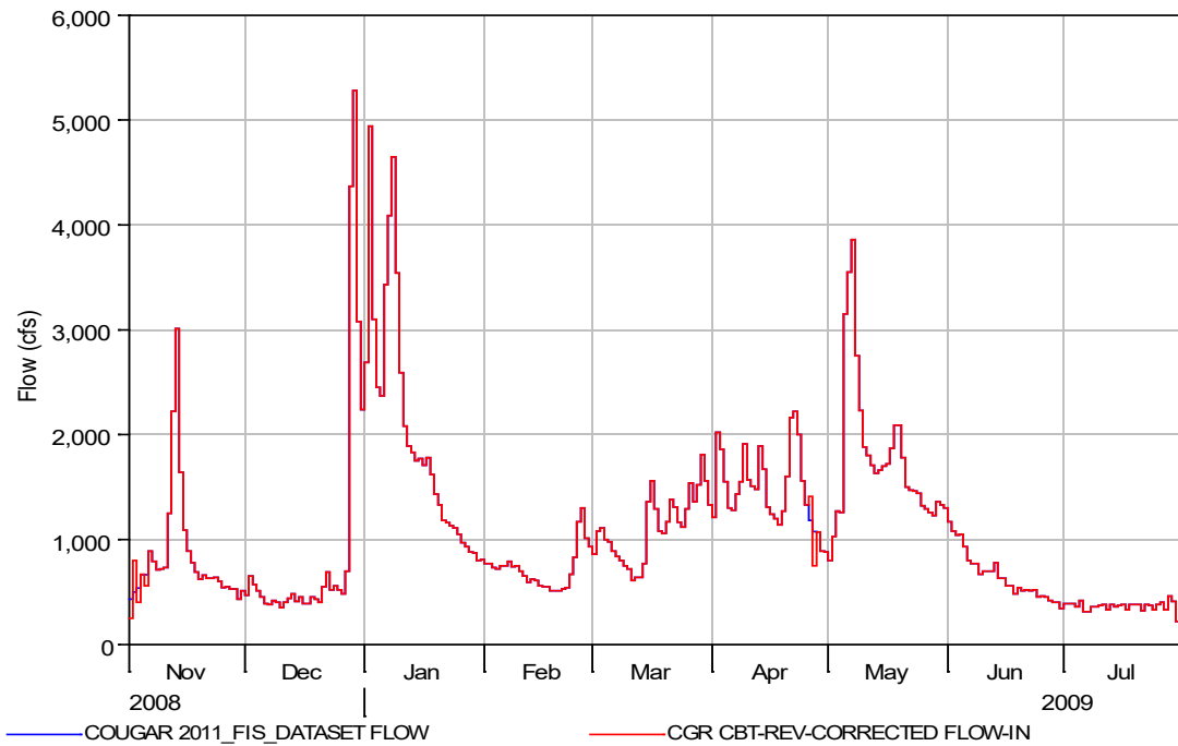
Figure 2-24. Water Year 2009 Comparison at Cougar Reservoir.
