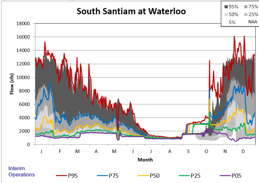
Figure 5-228. Waterloo Updated Interim Operations Non-exceedance Plot.
