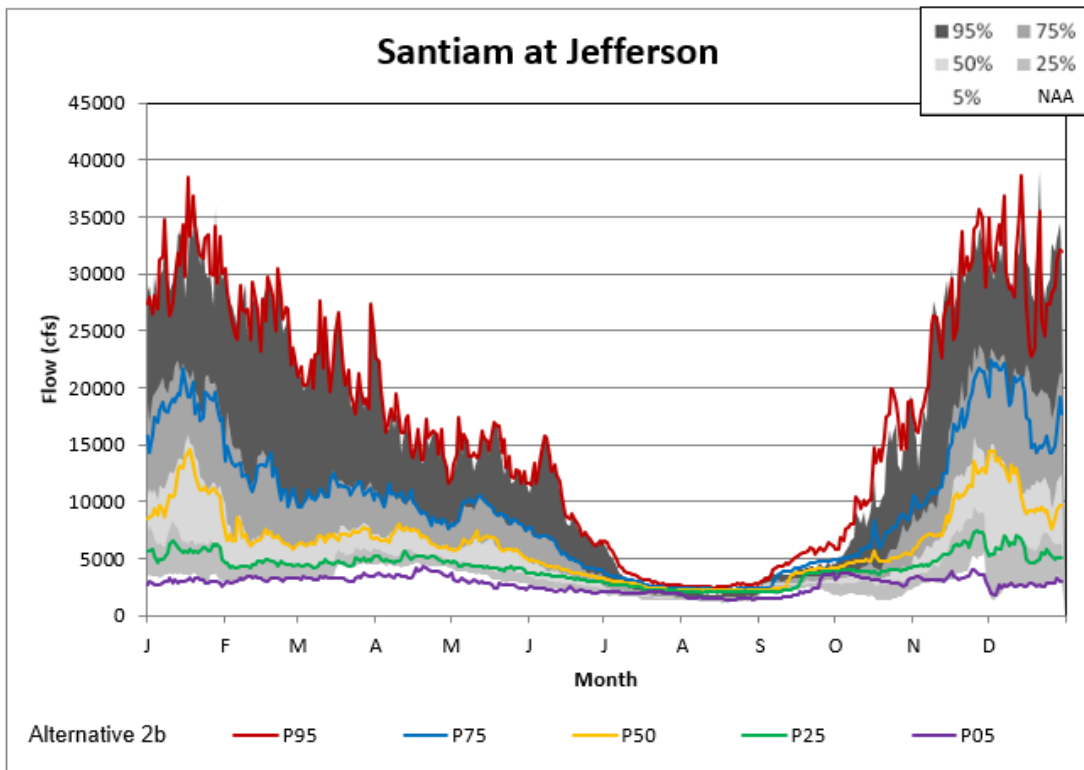
Figure 5-66. Jefferson Alternative 2B Non-exceedance Plot.
