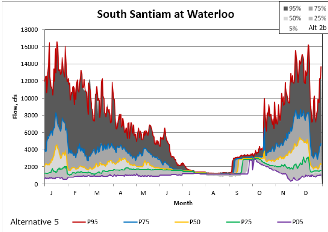
Figure 5-251. Waterloo Alternatives 5/2B Non-exceedance Plot.
