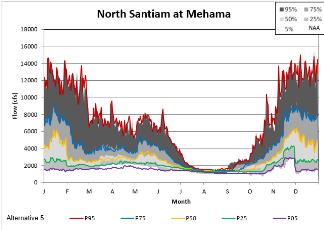
Figure 5-157. Mehama Alternative 5 Non-exceedance Plot.
