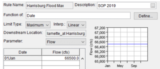
Figure 3-7. HEC-ResSim Screen Shots of Downstream Maximum Rules.
