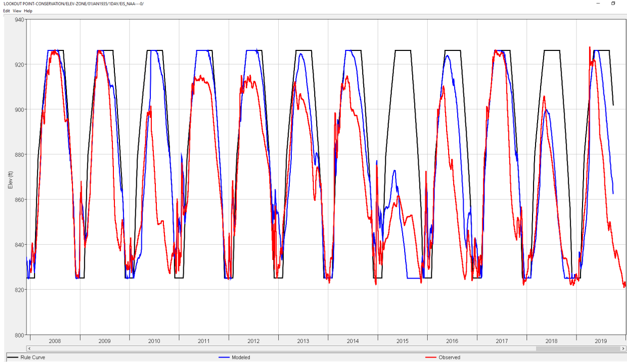
Figure 3-64. Lookout Point Dam and Reservoir Model Validation.
