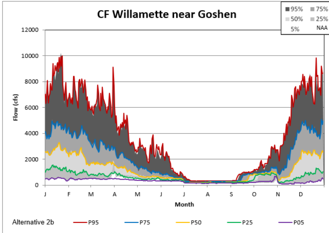
Figure 5-61. Goshen Alternative 2B Non-exceedance Plot.
