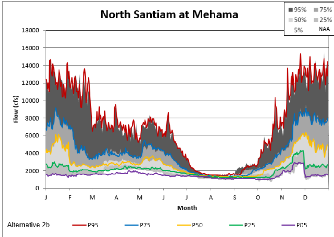
Figure 5-65. Mehama Alternative 2B Non-exceedance Plot.
