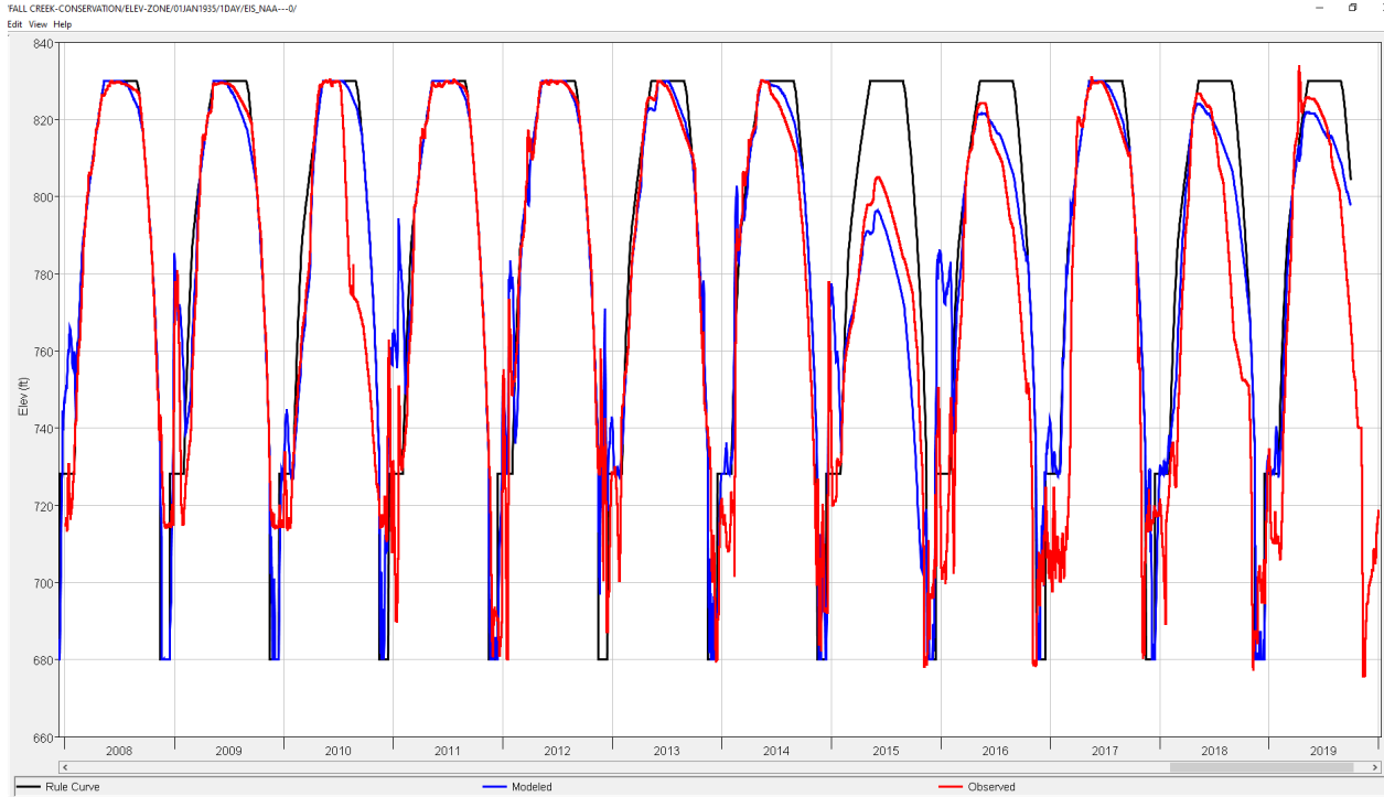
Figure 3-62. Fall Creek Dam and Reservoir Model Validation.
