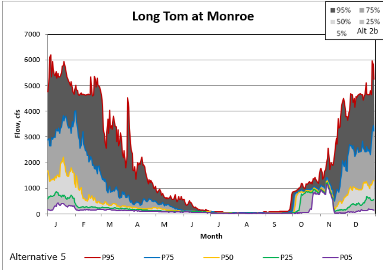
Figure 5-246. Monroe Alternatives 5/2B Non-exceedance Plot.
