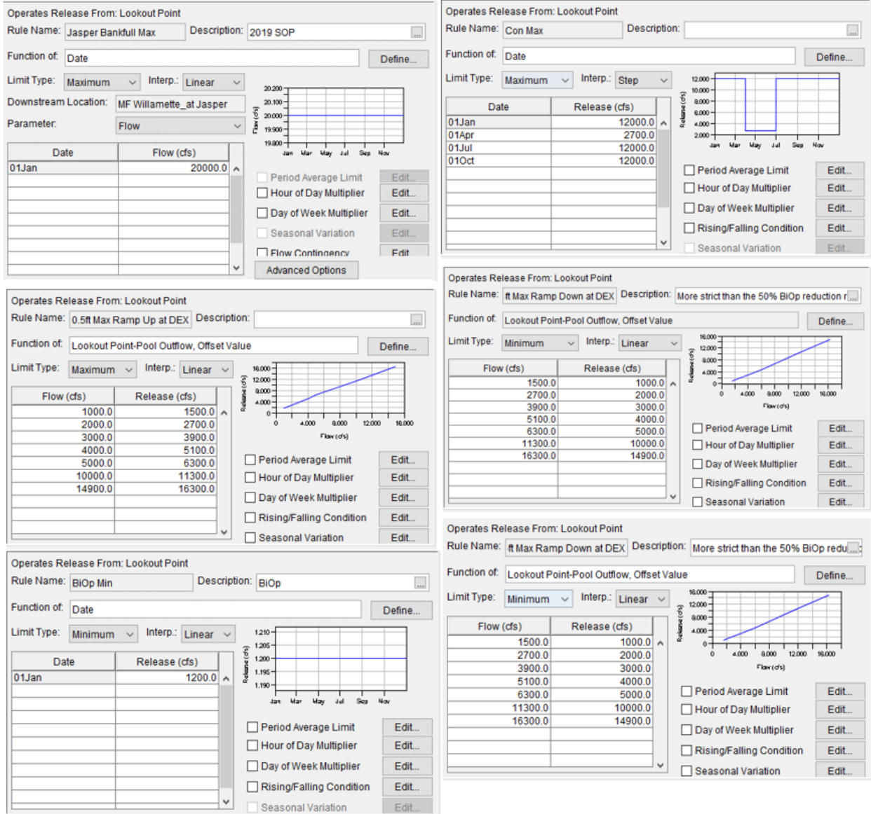
Figure 3-40. Lookout Point Dam and Reservoir NAA Operation Set Rules, Continued.
