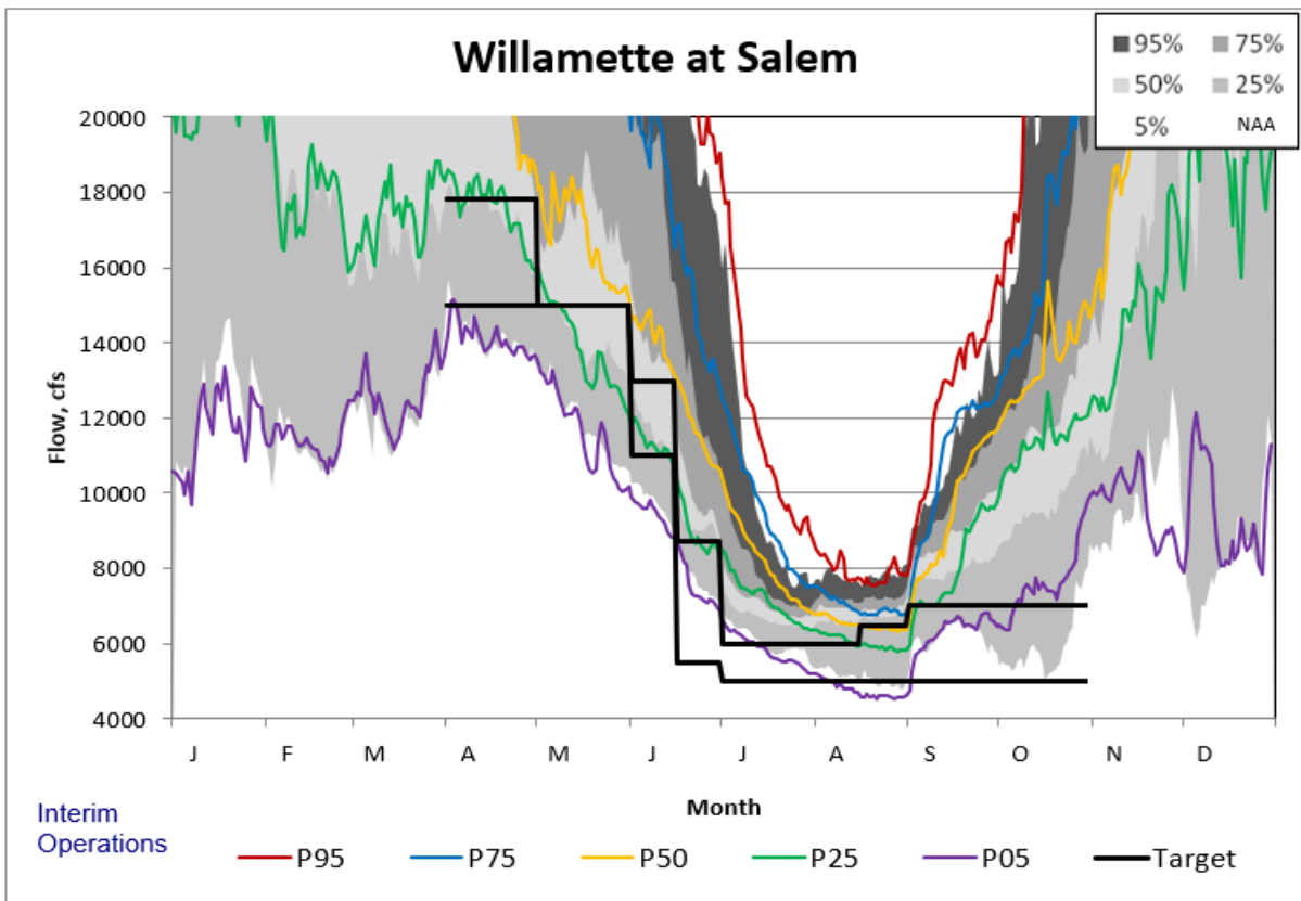
Figure 5-231. Salem Updated Interim Operations Non-exceedance Plot.
