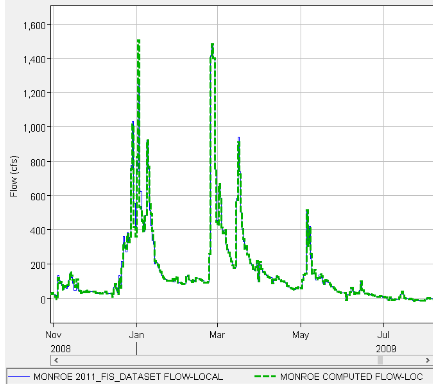
Figure 2-33. Water Year 2009 Comparison at Monroe, OR.
