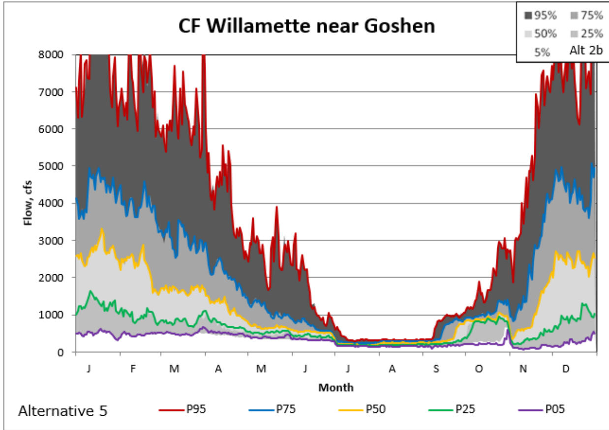
Figure 5-245. Goshen Alternatives 5/2B Non-exceedance Plot.
