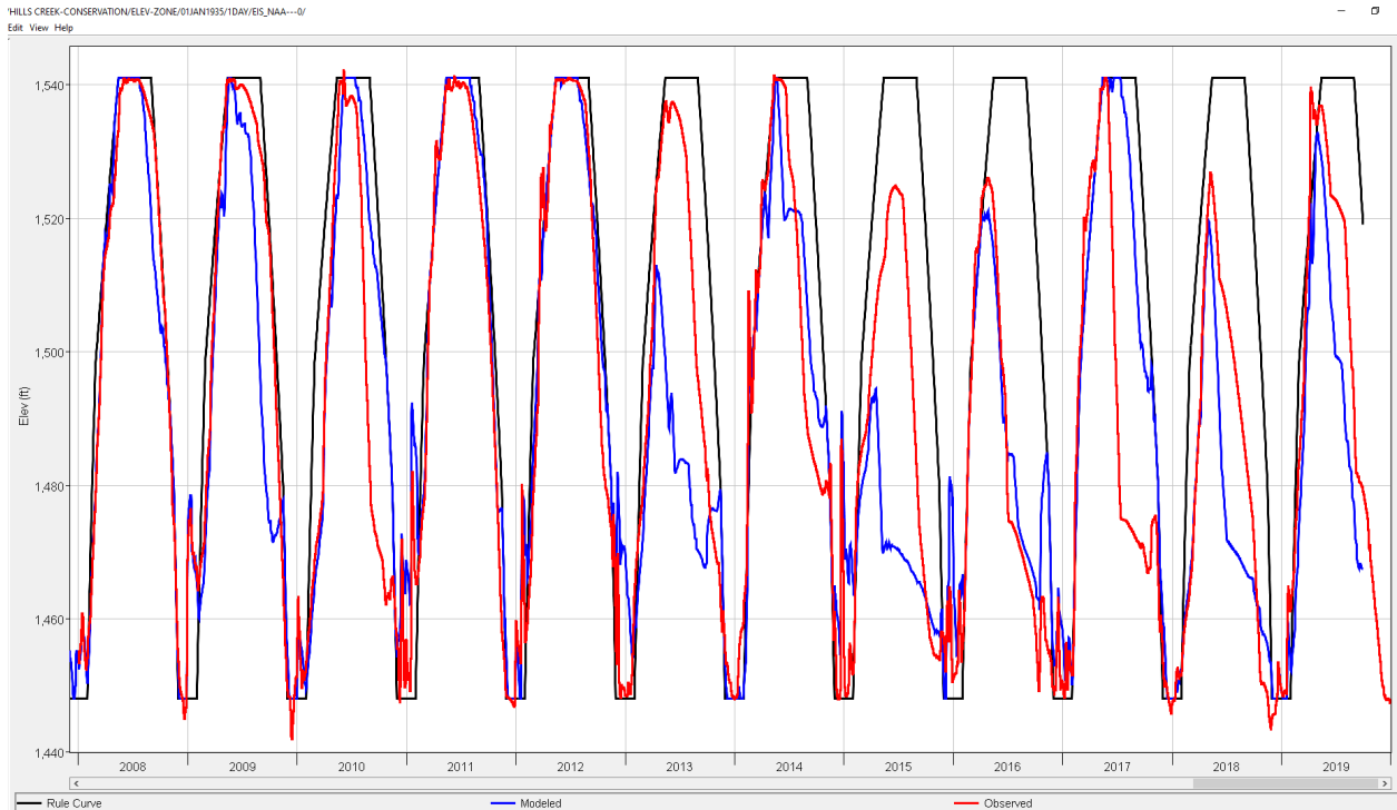
Figure 3-63. Hills Creek Dam and Reservoir Model Validation.
