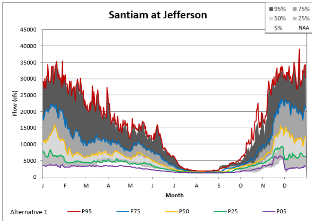
Figure 5-20. Jefferson Alternative 1 Non-exceedance Plot.
