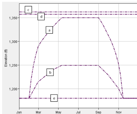
Figure 3-12. Blue River Dam and Reservoir HEC-ResSim Water Control Diagram.
