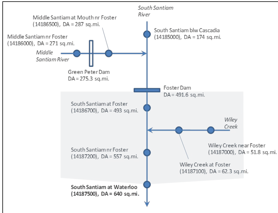
Figure 2-10. Waterloo Routing Diagram.
