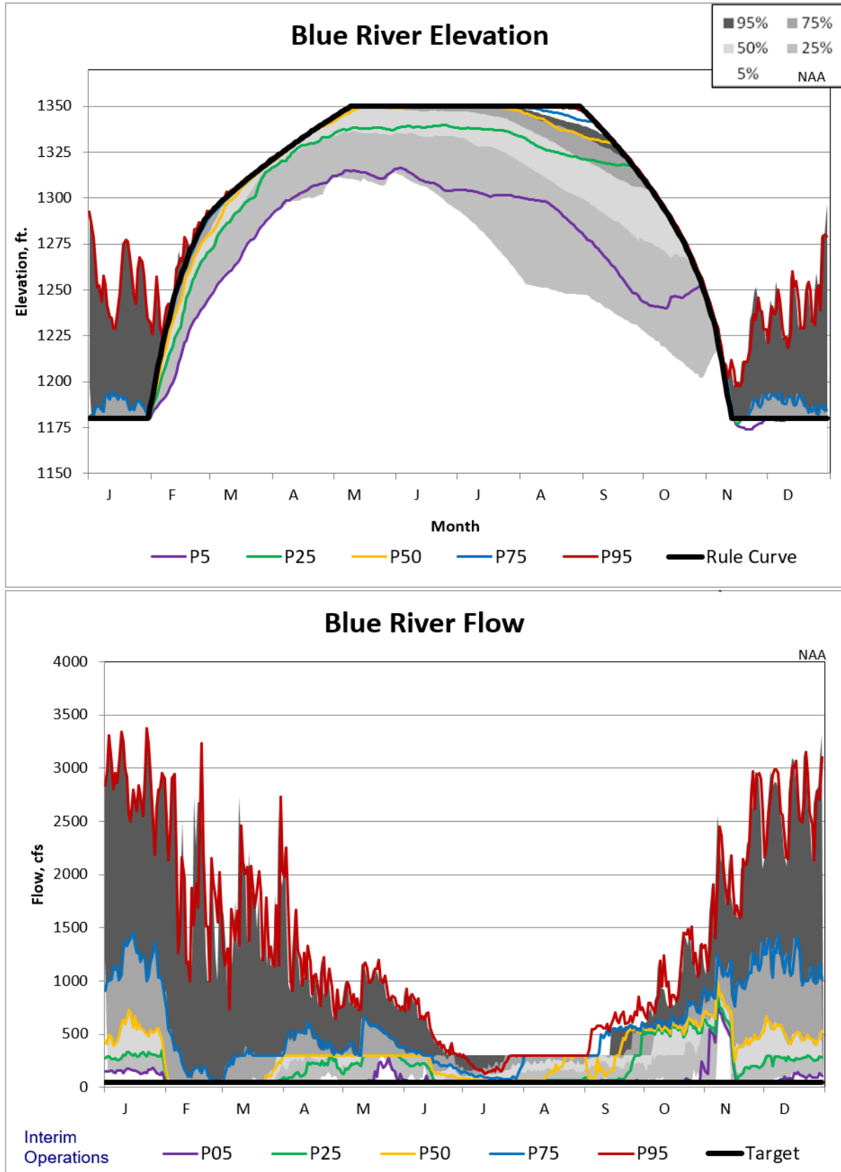
Figure 5-210. Blue River Updated Interim Operations Non-exceedance Plot.
