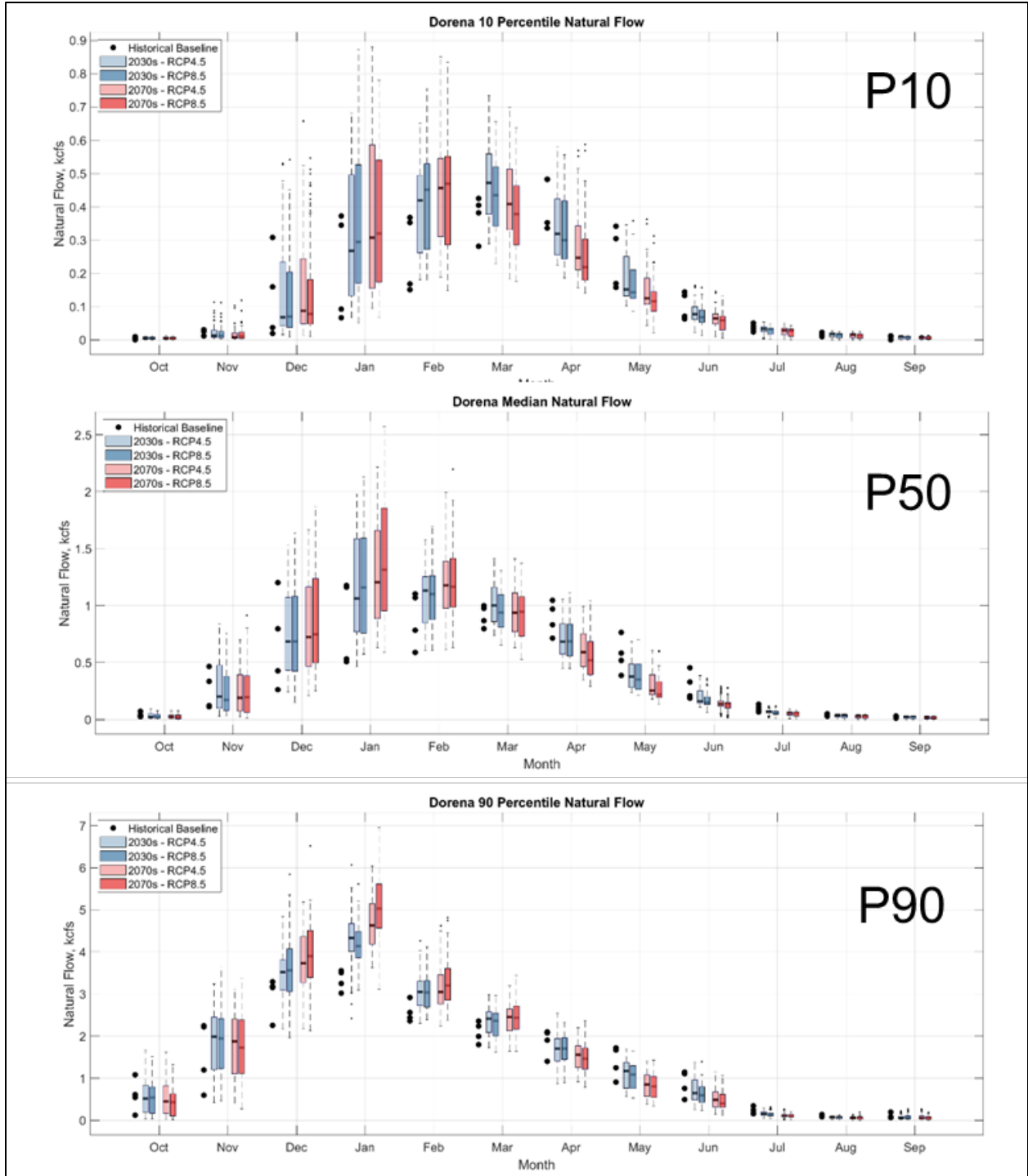
Figure 6-5. Dorena Dam and Reservoir Climate Change Projections.
