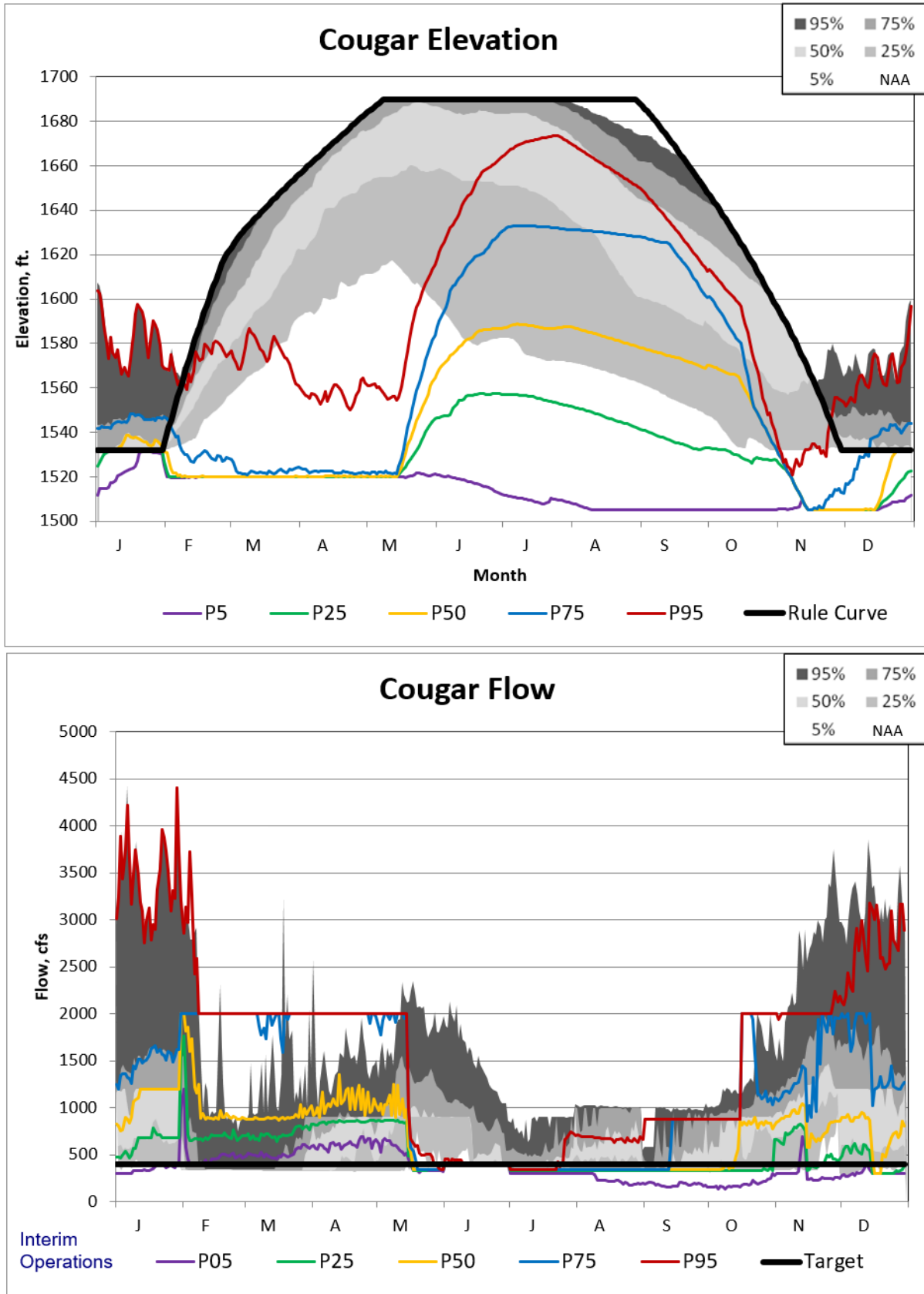
Figure 5-212. Cougar Updated Interim Operations Non-exceedance Plot.
