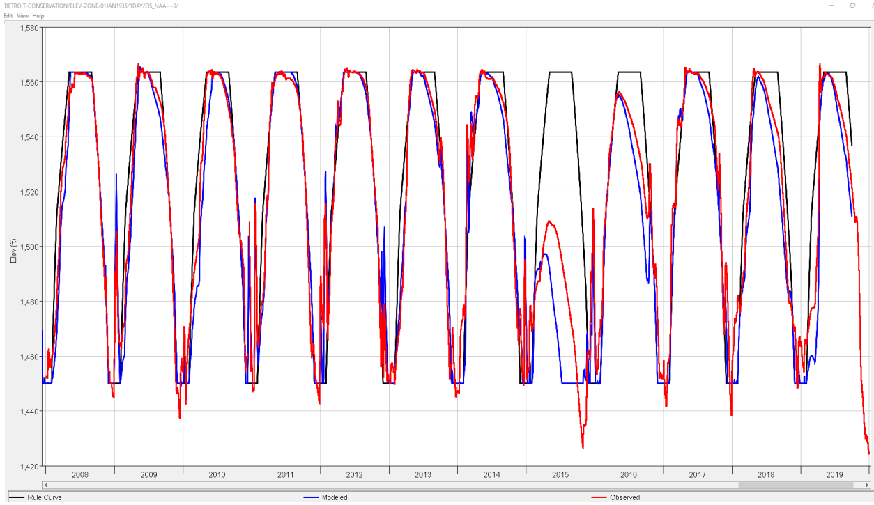
Figure 3-68. Detroit Dam and Reservoir Model Validation.
