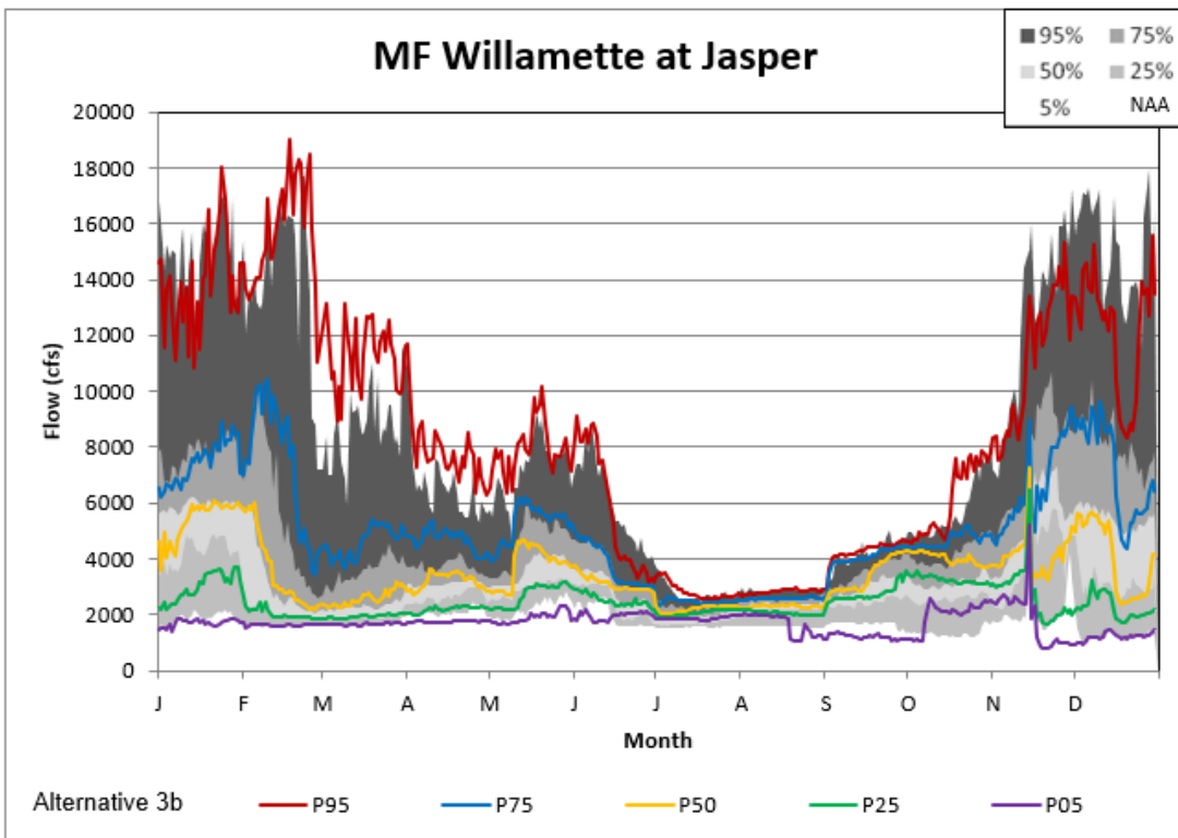
Figure 5-110. Jasper Alternative 3B Non-exceedance Plot.
