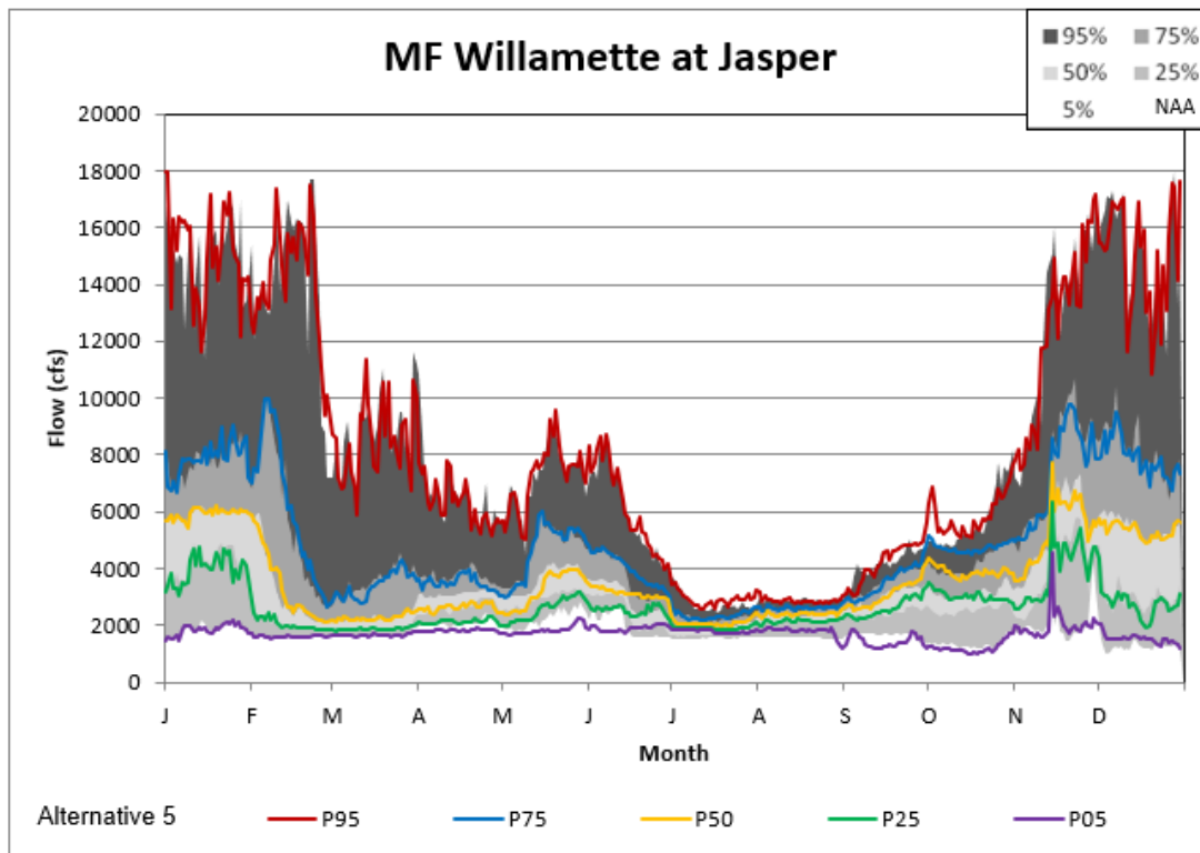
Figure 5-156. Jasper Alternative 5 Non-exceedance Plot.
