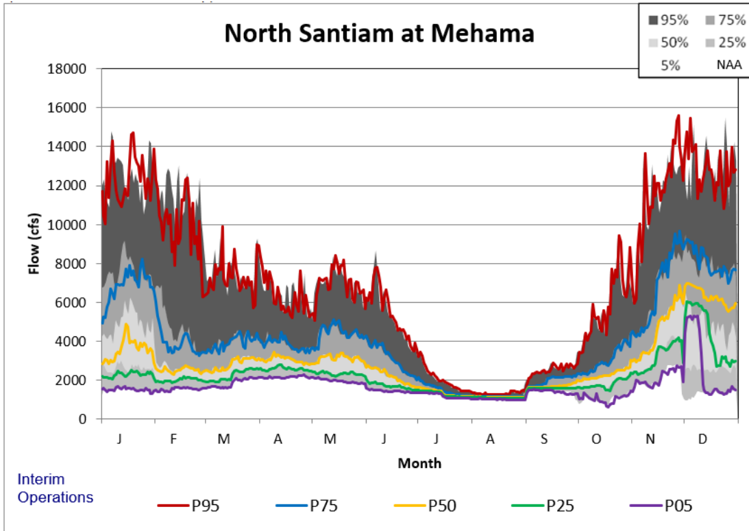
Figure 5-226. Mehama Updated Interim Operations Non-exceedance Plot.
