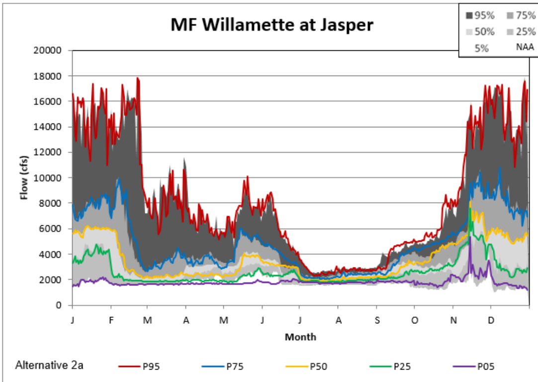
Figure 5-41. Jasper Alternative 2A Non-exceedance Plot.
