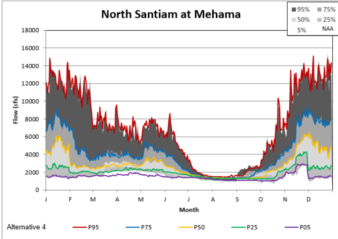
Figure 5-134. Mehama Alternative 4 Non-exceedance Plot.
