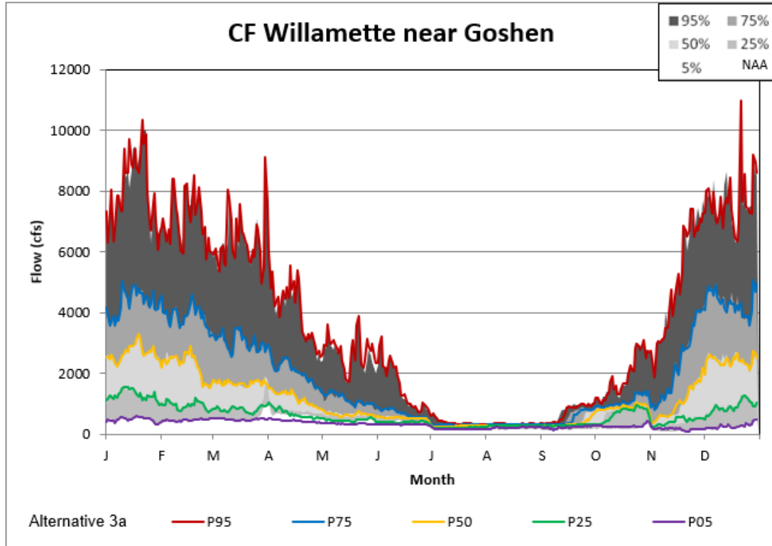
Figure 5-84. Goshen Alternative 3A Non-exceedance Plot.
