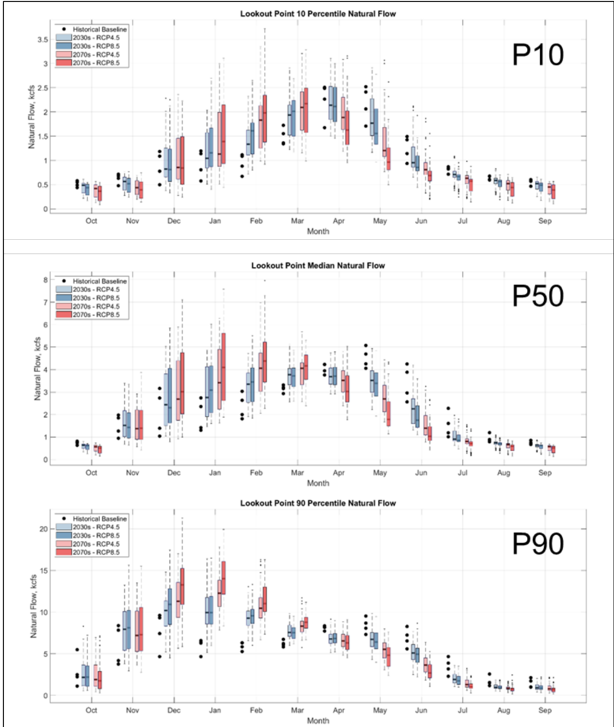
Figure 6-10. Lookout Point Dam and Reservoir Climate Change Projections.
