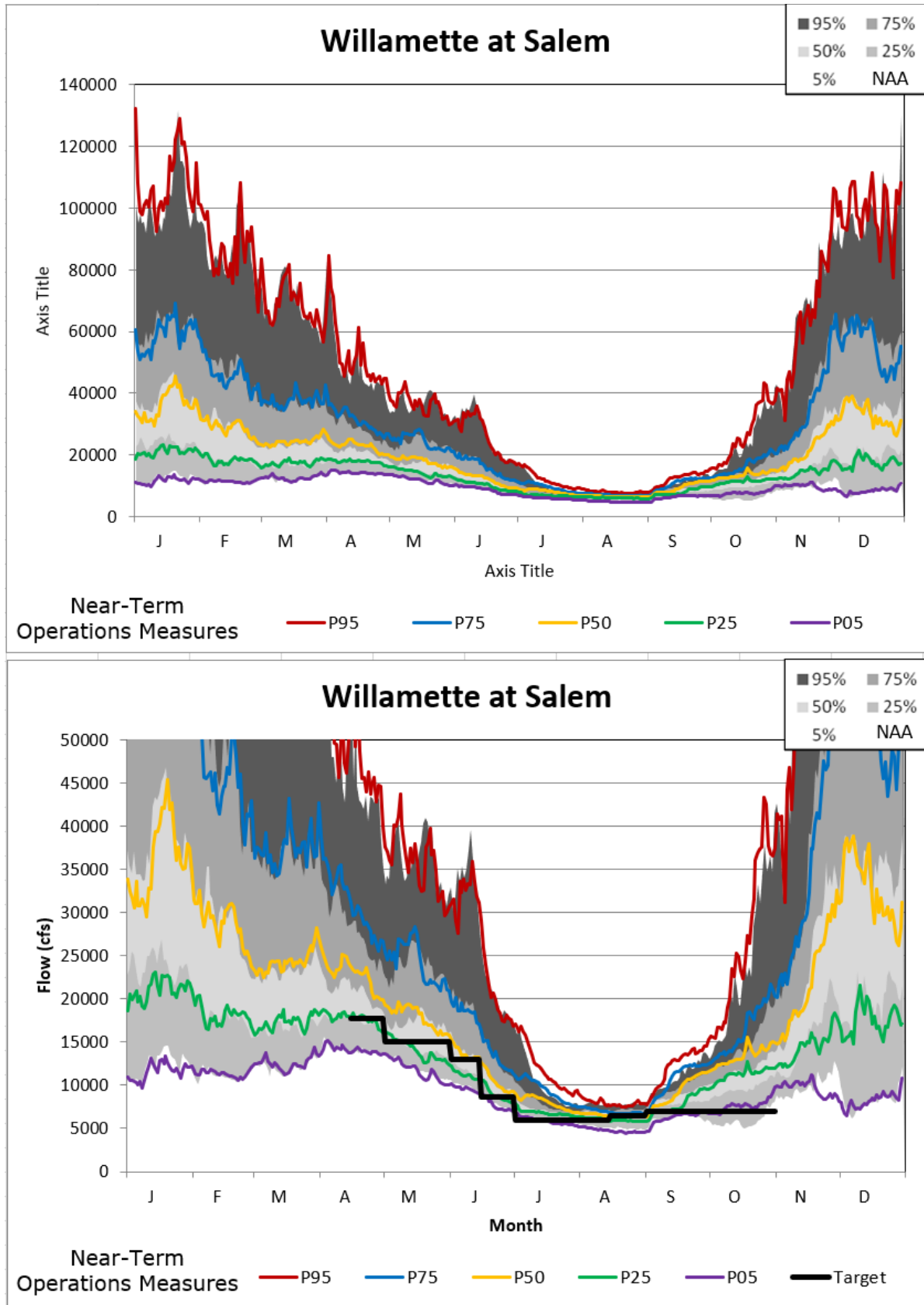
Figure 5-208. Salem Interim Operations Non-exceedance Plot.
