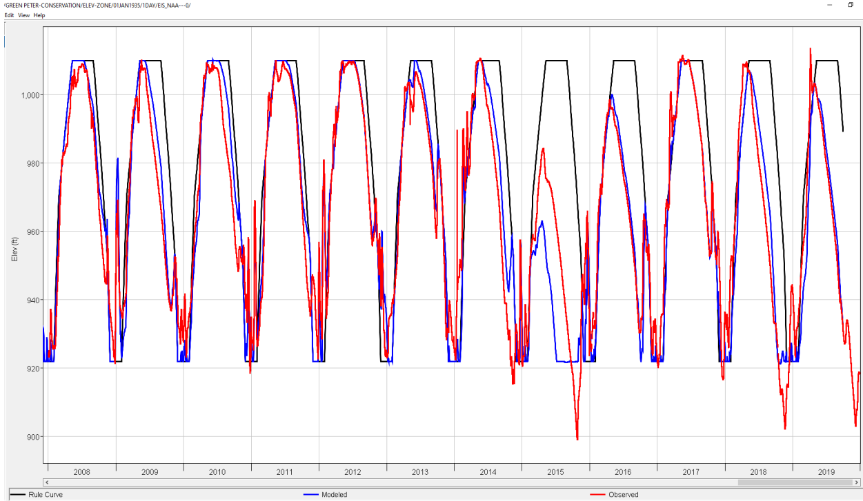
Figure 3-66. Green Peter Dam and Reservoir Model Validation.
