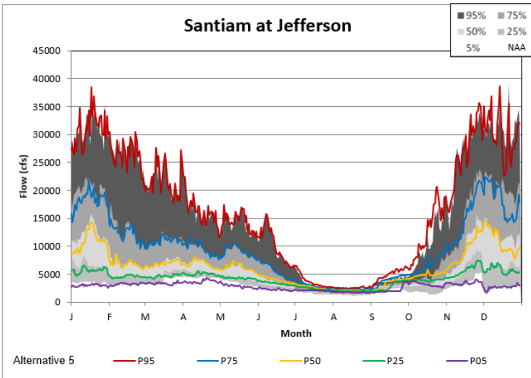
Figure 5-158. Jefferson Alternative 5 Non-exceedance Plot.
