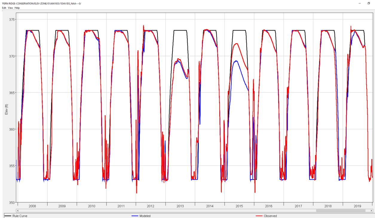
Figure 3-65. Fern Ridge Dam and Reservoir Model Validation.
