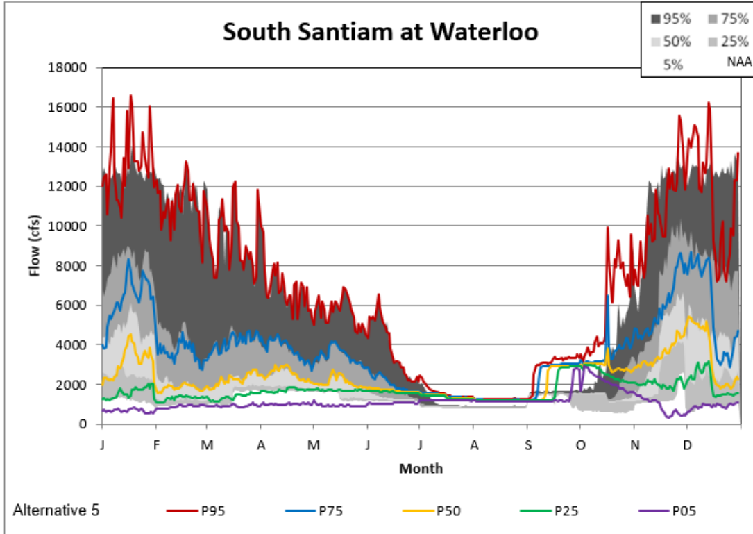
Figure 5-159. Waterloo Alternative 5 Non-exceedance Plot.
