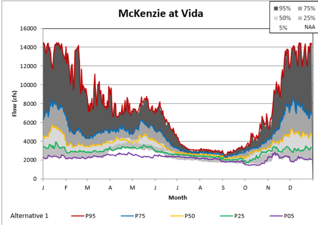
Figure 5-17. Vida Alternative 1 Non-exceedance Plot.
