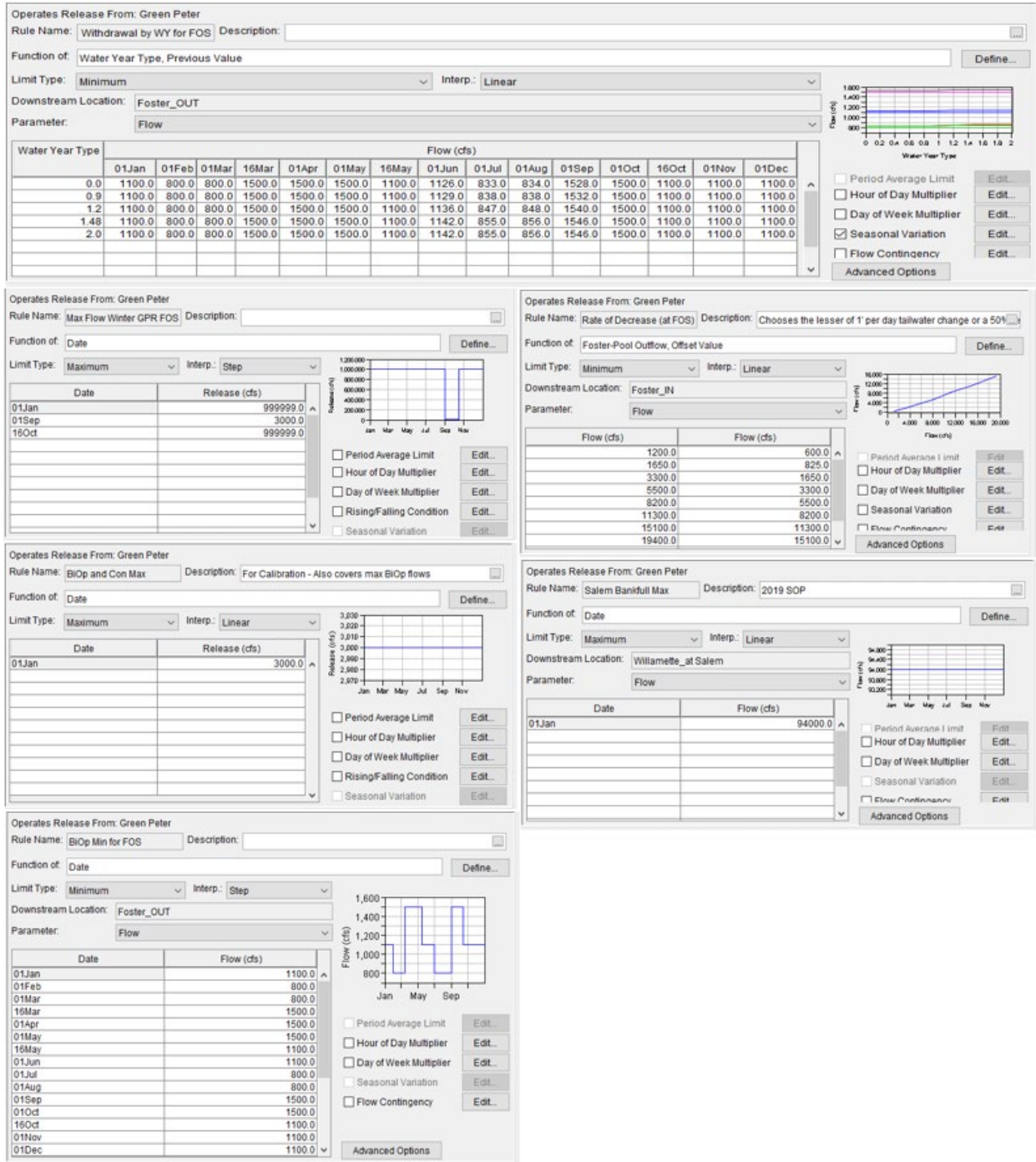
Figure 3-48. Green Peter Dam and Reservoir NAA Operation Set Rules, Continued.
