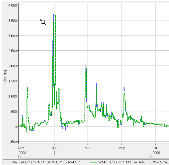
Figure 2-30. Water Year 2009 Comparison at Mehama, OR.
