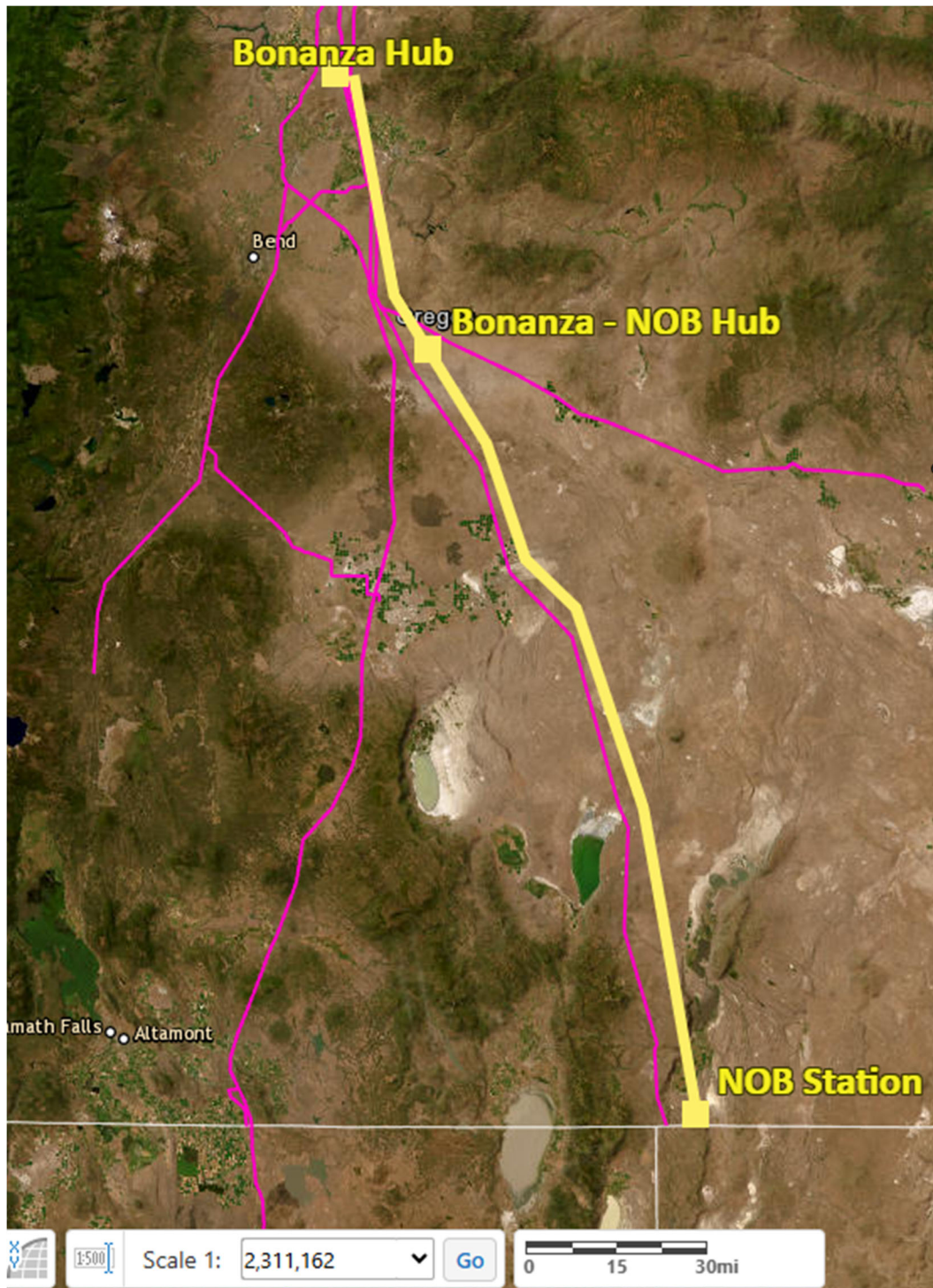
Figure 10.2: Estimated route for BZNA-POI-NOB 500 kV circuits
