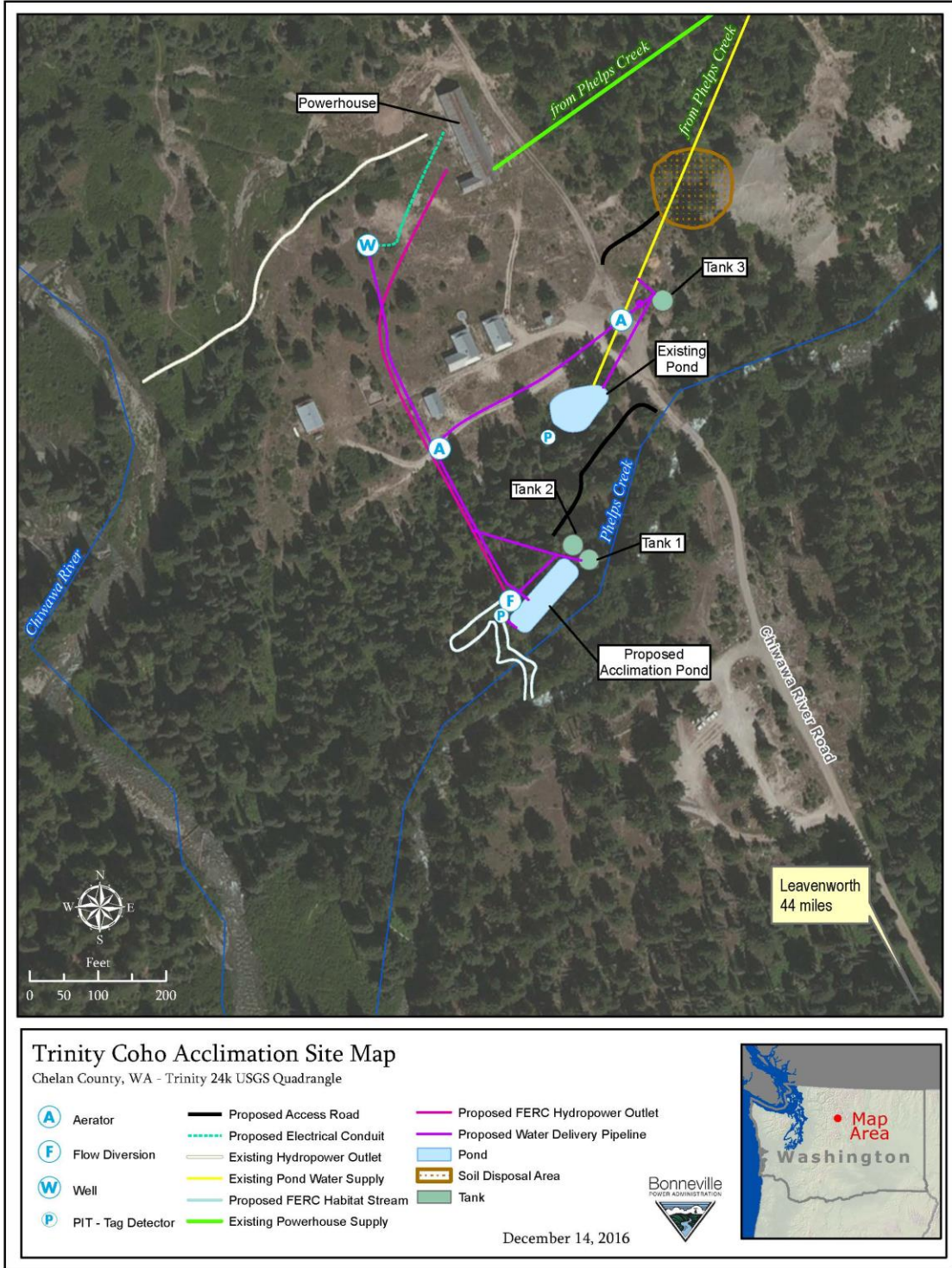
Figure 1. Trinity Coho Acclimation Facility Site Plan
