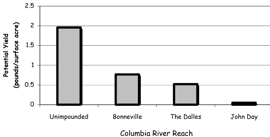
Figure 1: Potential sustainable harvest for white sturgeon in the Columbia River downstream from Bonneville Dam (unimpounded) and in the three reservoirs immediately upstream. Potential yield is estimated from area-specific annual recruitment, growth rates, and natural mortality. 3
